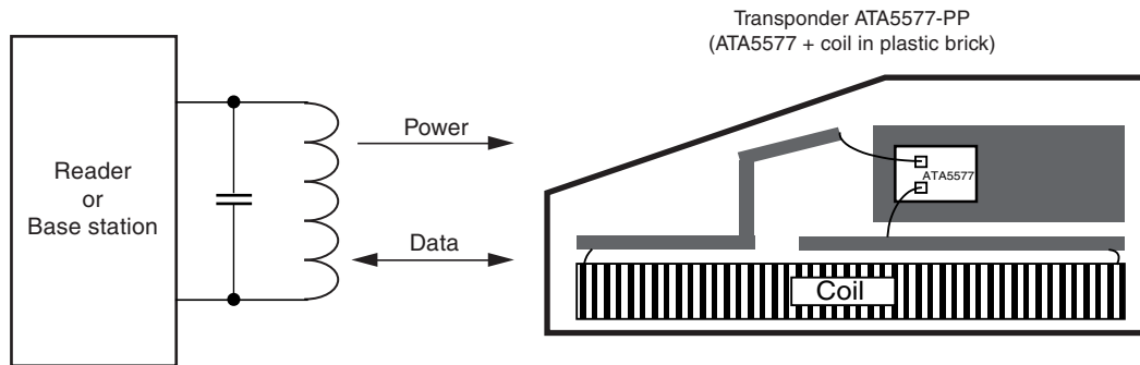
Figure 1-1. RFID System Using Atmel ATA5577M1-PP Transponder
