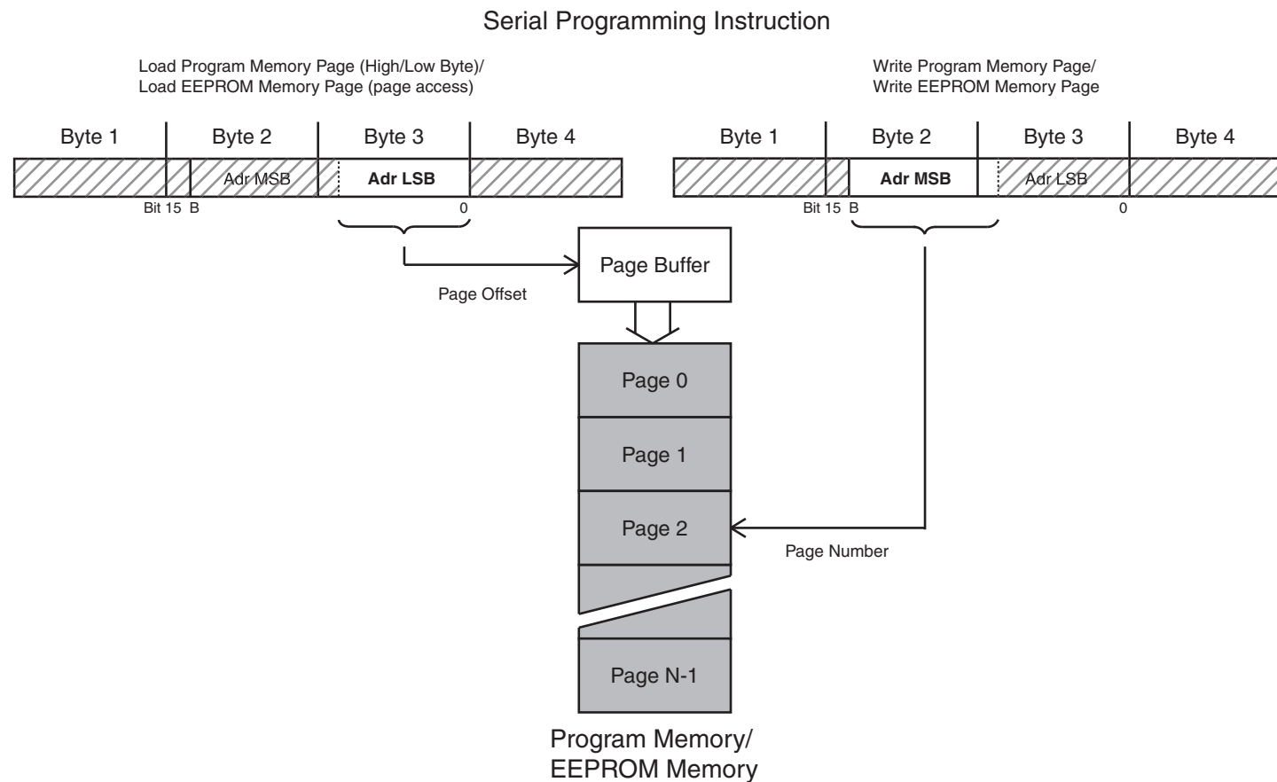
Figure 28-2. Serial Programming Instruction example
