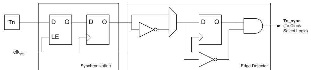
Figure 22-1. T 0 Pin Sampling
