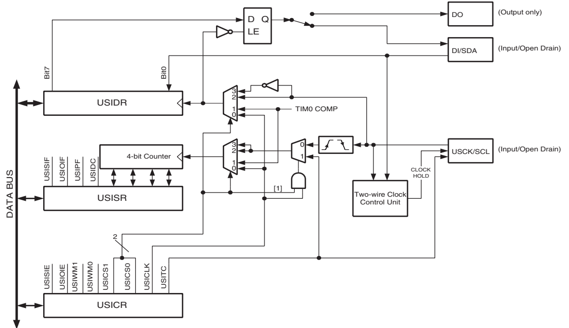
Figure 23-1. Universal Serial Interface, Block Diagram
