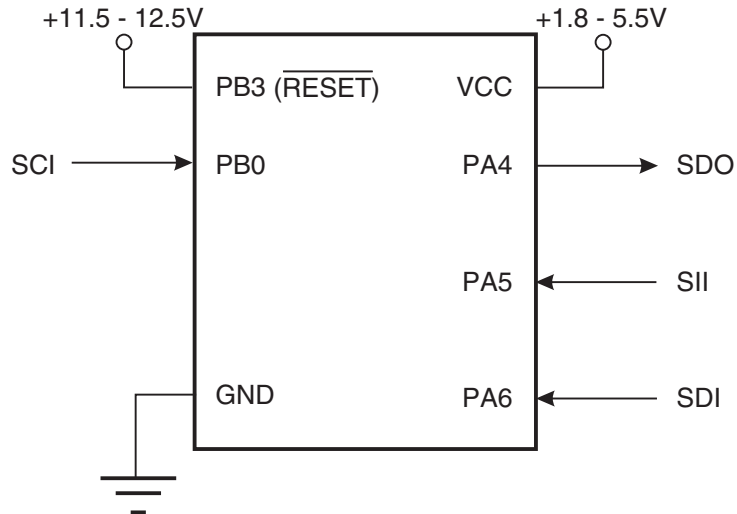
Figure 28-3. High-voltage Serial Programming
