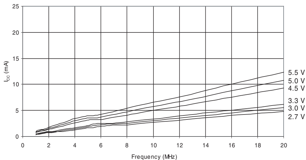
Figure 30-4. Active Supply Current vs. frequency (1 - 20 MHz) - Temp.=125°C
