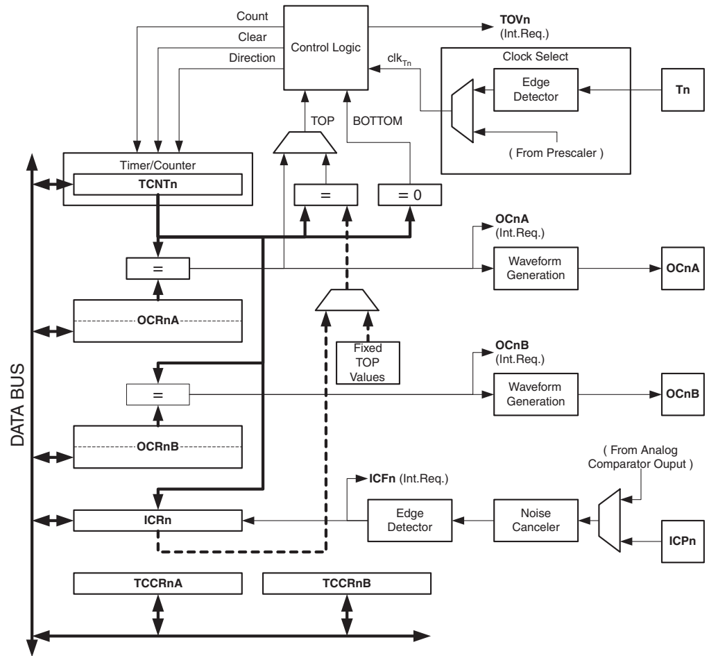
Figure 21-1. 16-bit Timer/Counter Block Diagram
