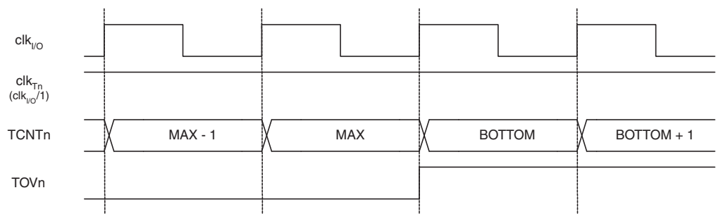
Figure 20-8. Timer/Counter Timing Diagram, no Prescaling
