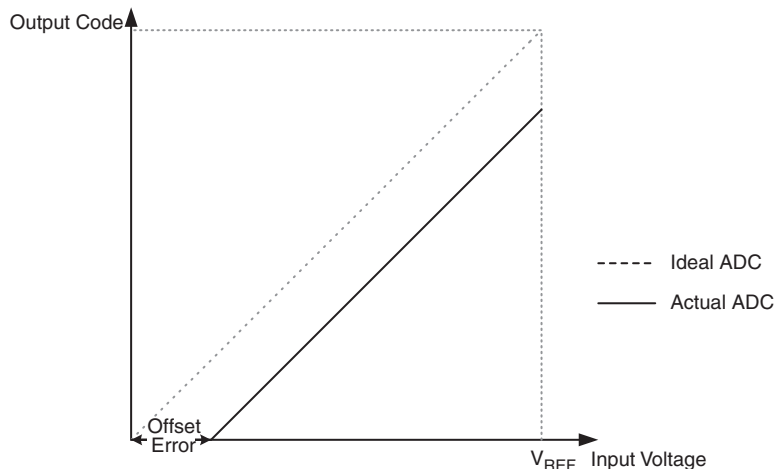
Figure 25-9. Offset Error
