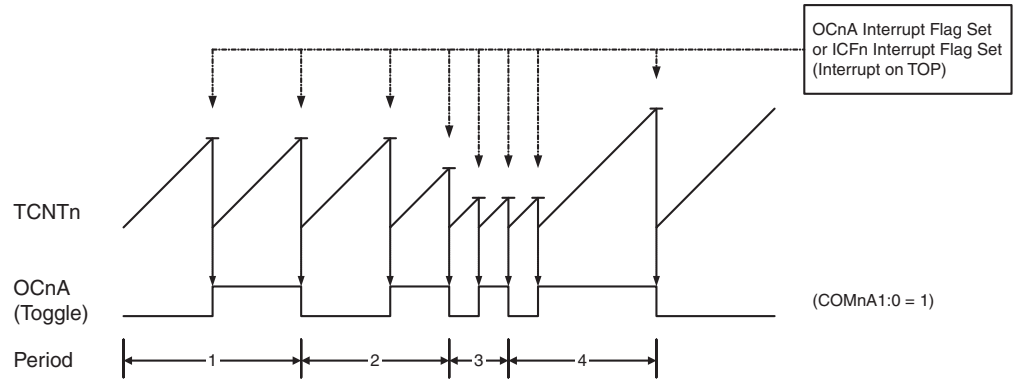
Figure 21-6. CTC Mode, Timing Diagram
