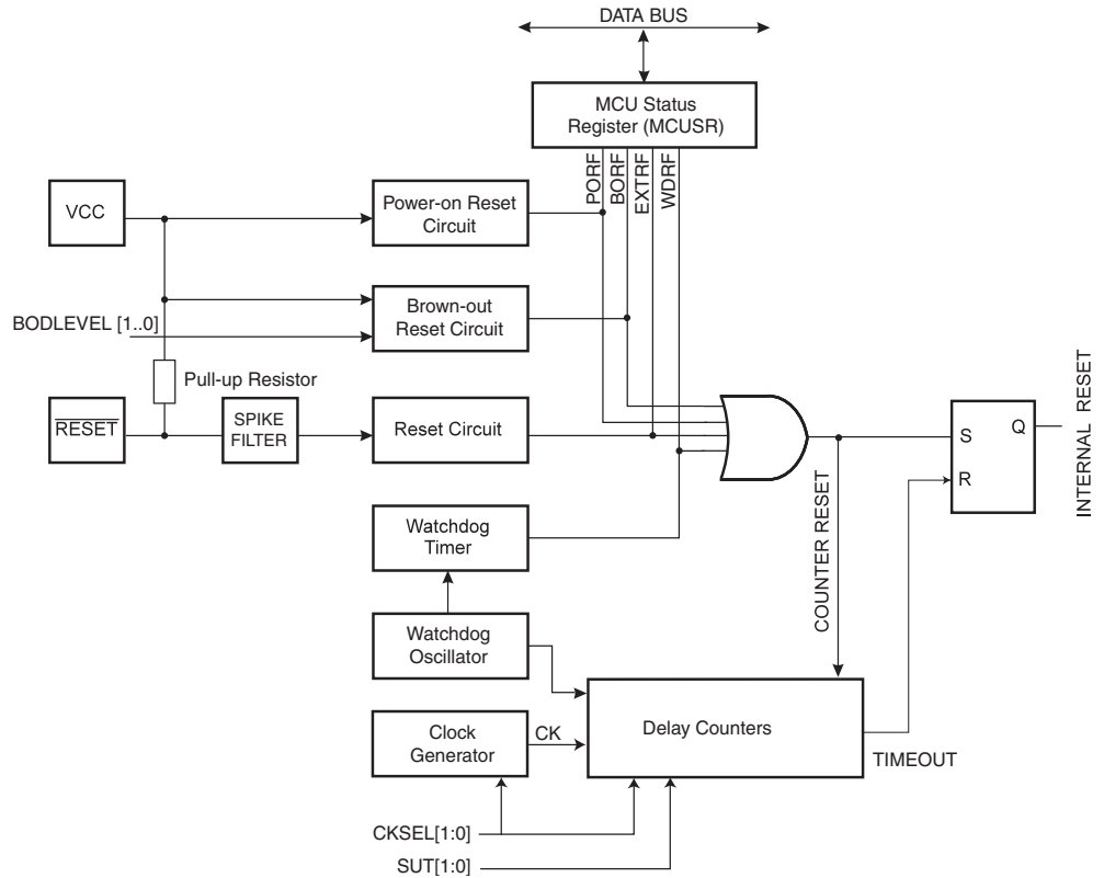
Figure 16-1. Reset Logic
