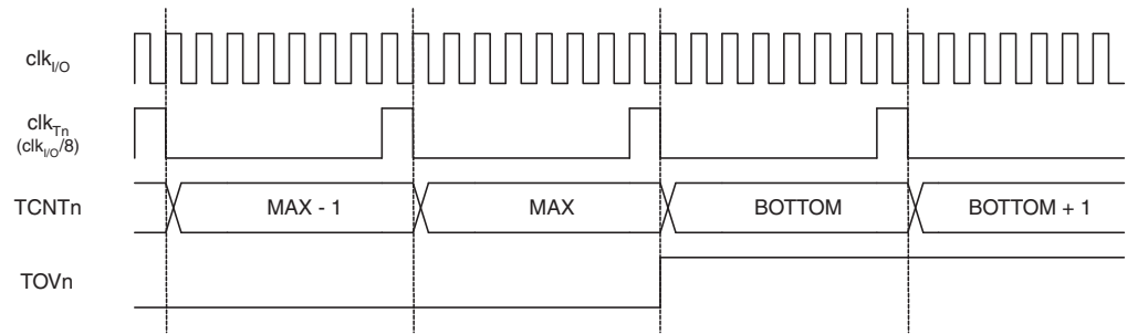
Figure 20-9. Timer/Counter Timing Diagram, with Prescaler ( f_{clk\_I/O}/8 )
