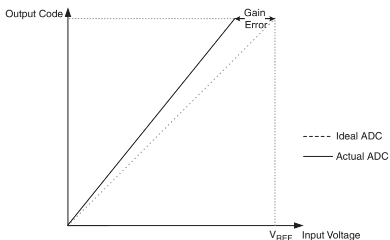
Figure 25-10. Gain Error
