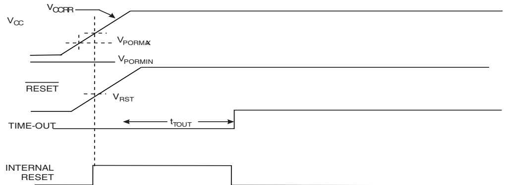
Figure 16-2. MCU Start-up, \overline{\text{RESET}} Tied to V_{CC}
