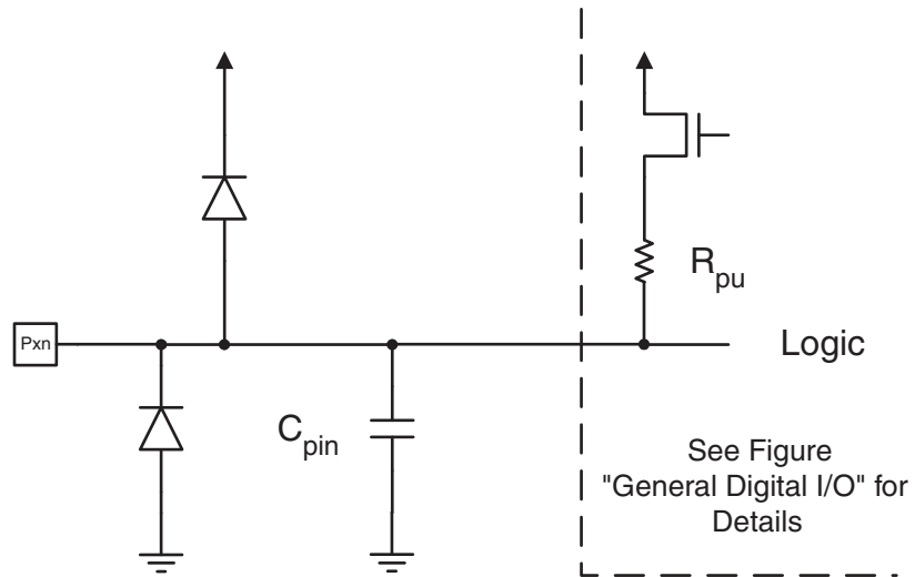
Figure 19-1. I/O Pin Equivalent Schematic
