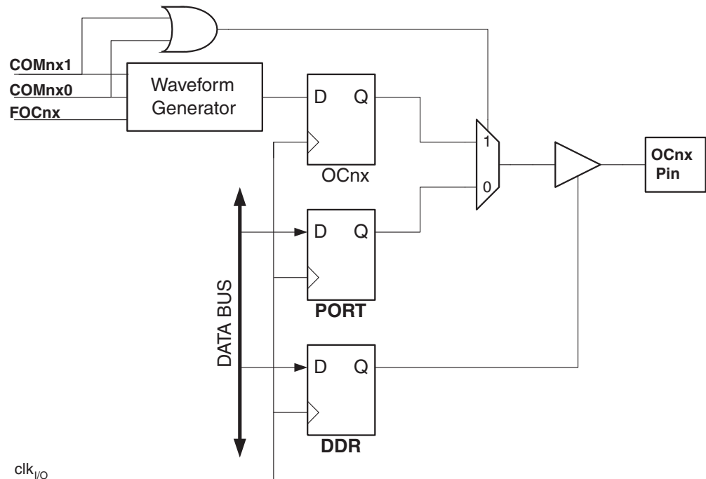
Figure 21-5. Compare Match Output Unit, Schematic
