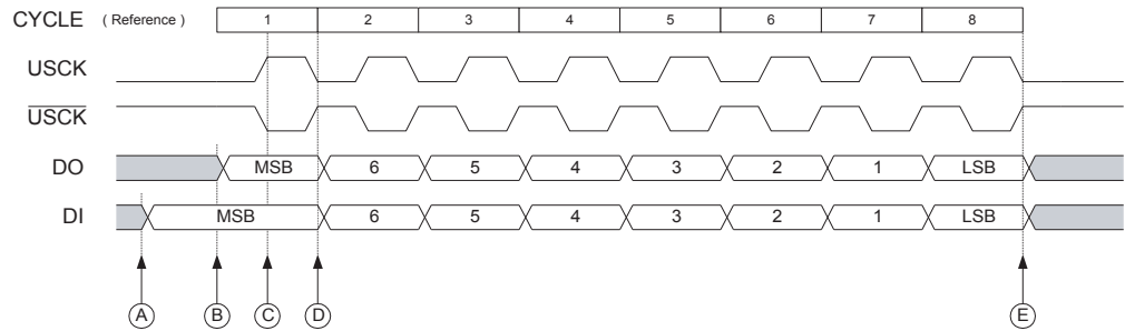
Figure 23-3. Three-wire Mode, Timing Diagram
