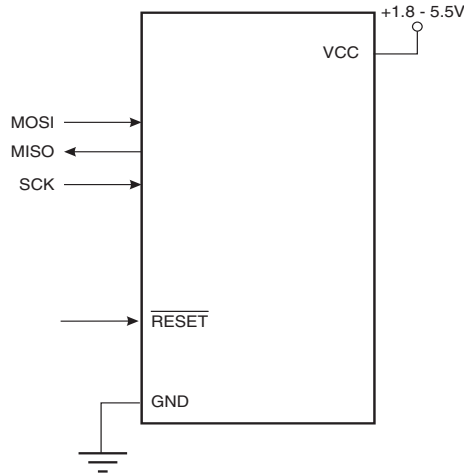
Figure 28-1. Serial Programming and Verify (1)
