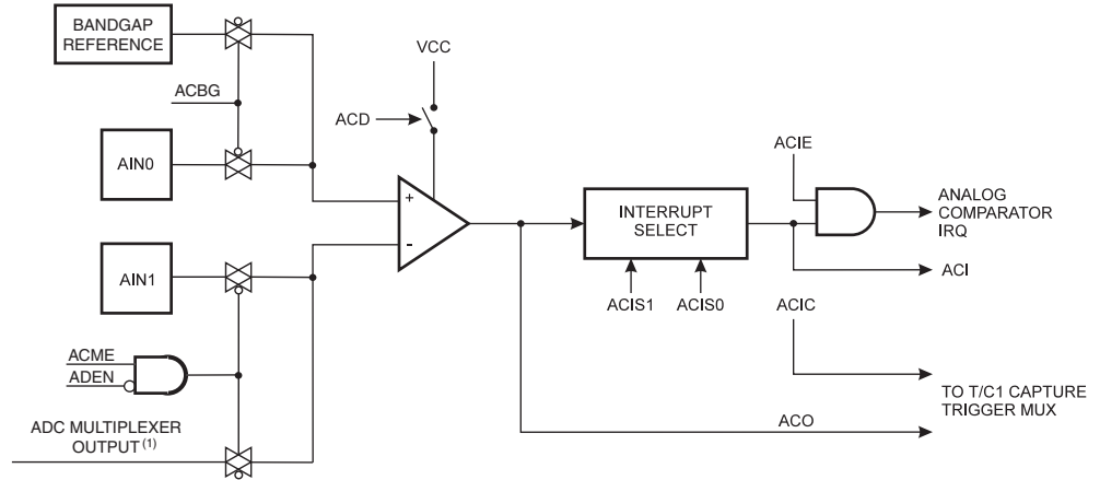
Figure 24-1. Analog Comparator Block Diagram (1)
