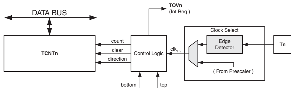
Figure 20-2. Counter Unit Block Diagram
