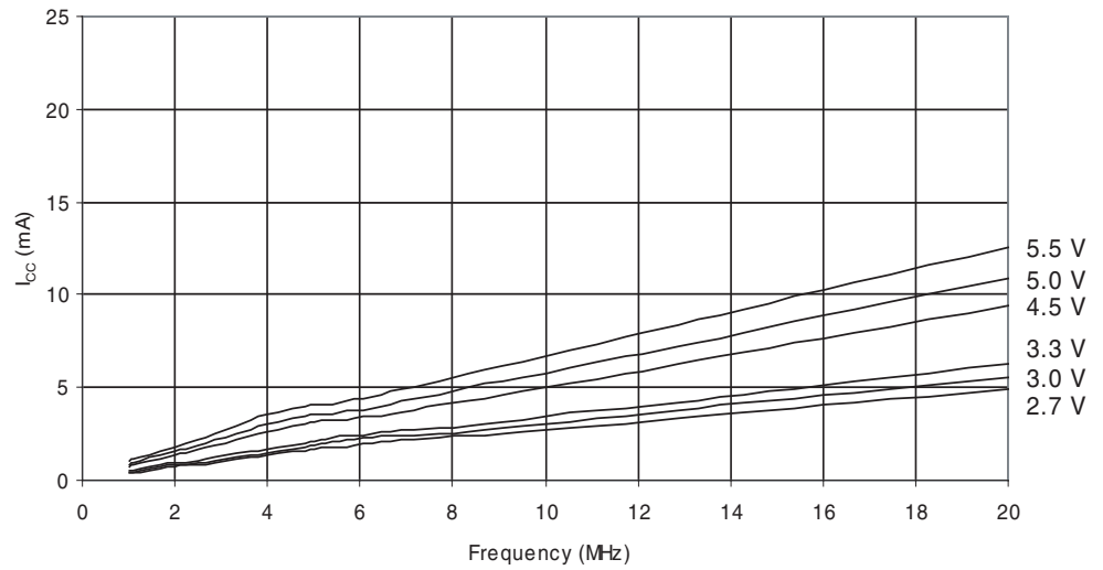
Figure 30-5. Active Supply Current vs. V_{CC} (Internal RC Oscillator, 8 MHz)
