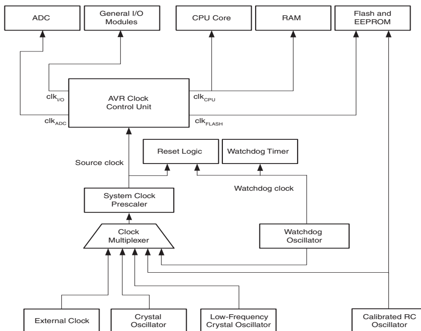
Figure 14-1. Clock Distribution
