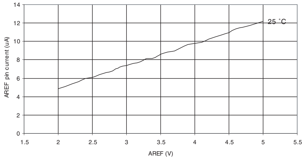
Figure 30-38. Analog Comparator Current vs. V_{CC}
