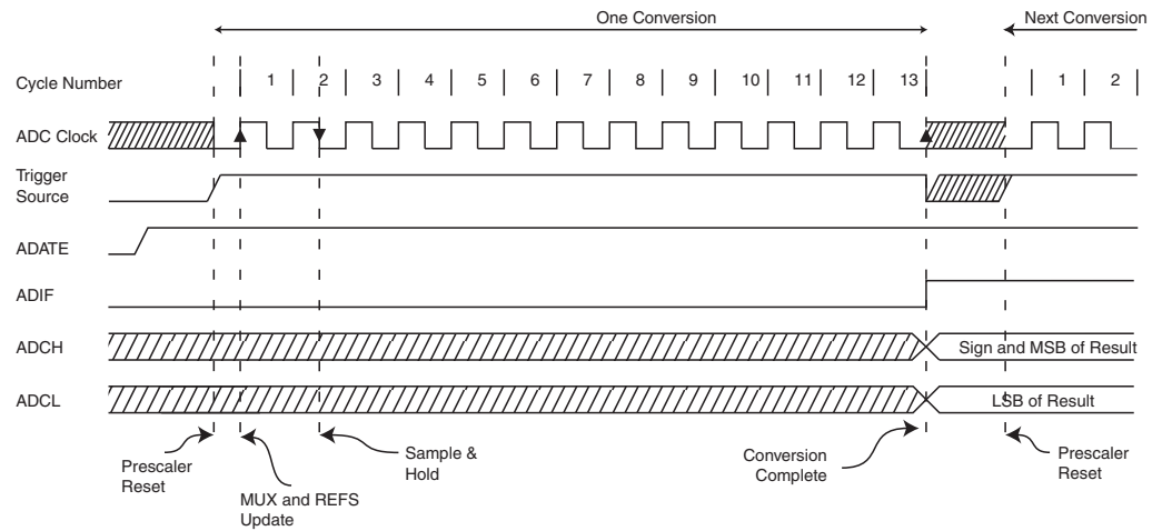
Figure 25-6. ADC Timing Diagram, Auto Triggered Conversion
