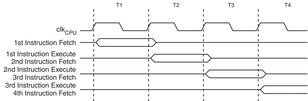
Figure 12-4. The Parallel Instruction Fetches and Instruction Executions
