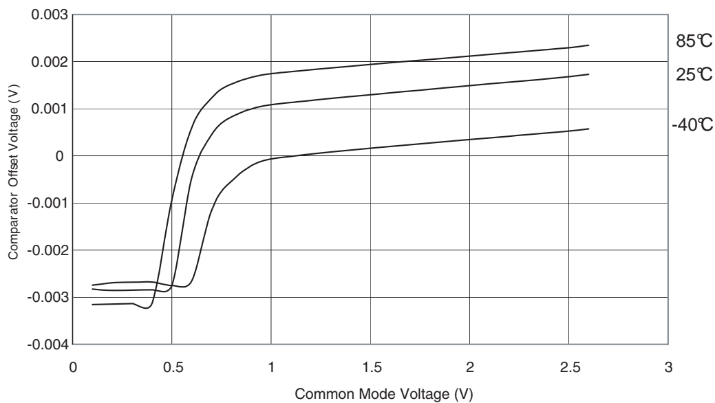
Figure 27-52. Analog Comparator Offset Voltage vs. Common Mode Voltage ( V_{CC} = 2.7V )
