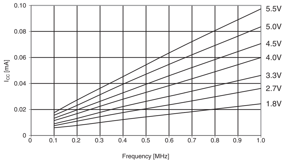
Figure 29-392. Atmel ATmega1284P: Reset supply current vs. low frequency (0.1 - 1.0MHz).
