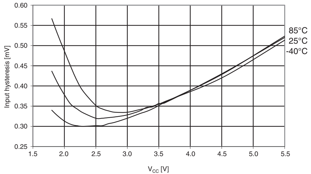
Figure 29-322. Atmel ATmega1284: I/O pin input hysteresis vs. V_{CC} .
