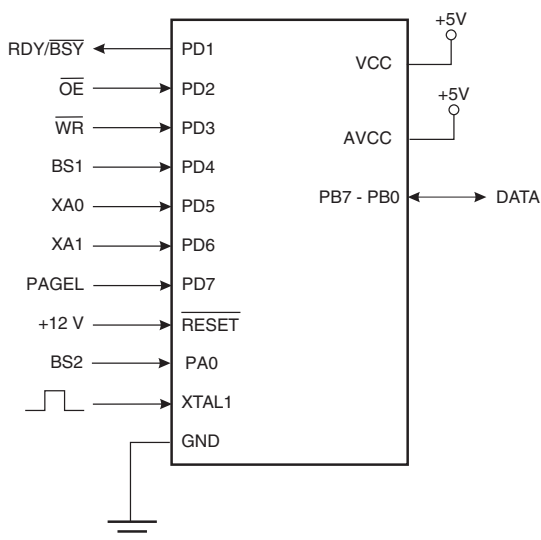
Figure 27-1. Parallel programming (1) .
