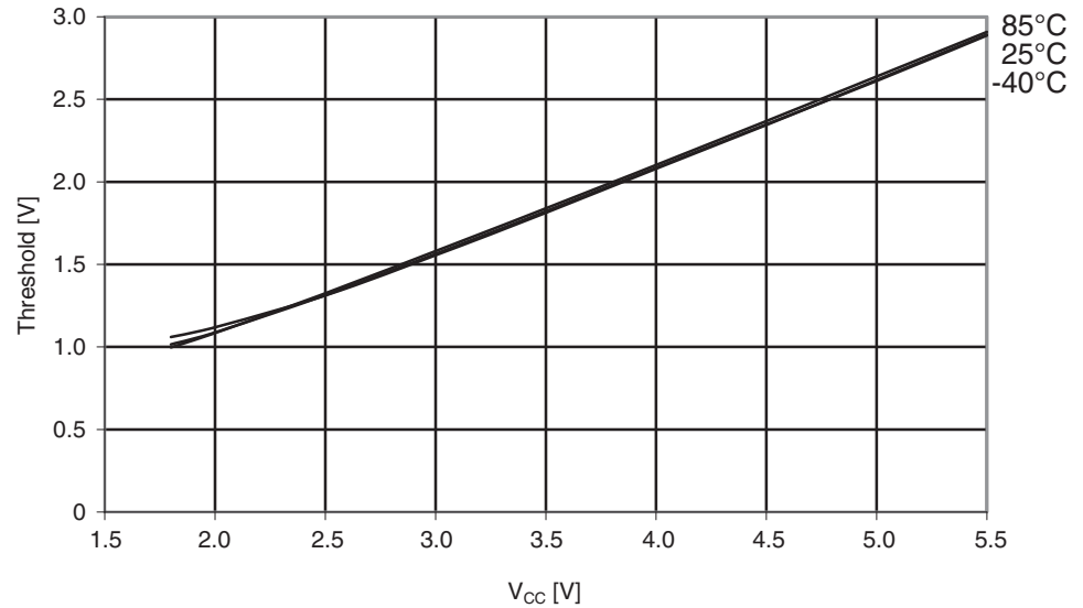
Figure 29-370. Atmel ATmega1284P: I/O pin input threshold vs. V_{CC} ( V_{IH} , I/O pin read as '1').
