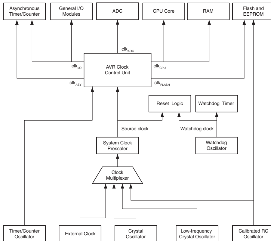
Figure 9-1. Clock distribution.
