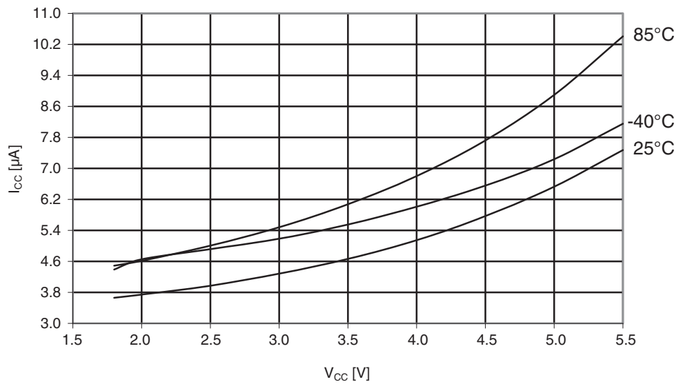
Figure 29-356. Atmel ATmega1284P: Power-down supply current vs. V_{CC} (watchdog timer enabled).
