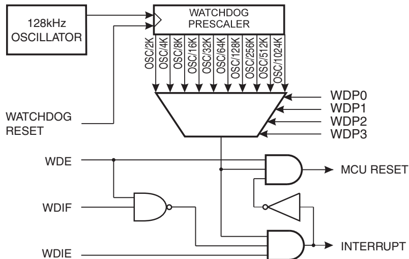
Figure 11-7. Watchdog Timer.
