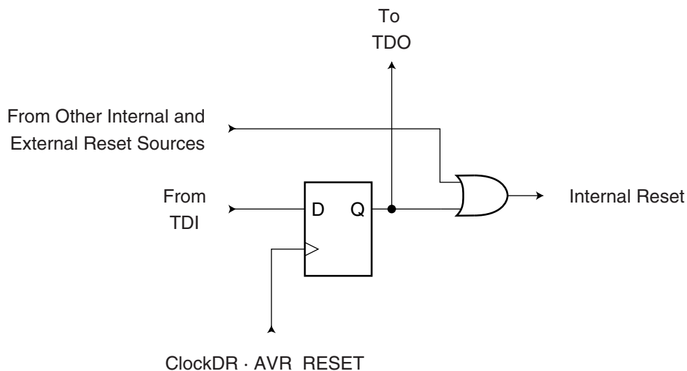
Figure 25-2. Reset Register
