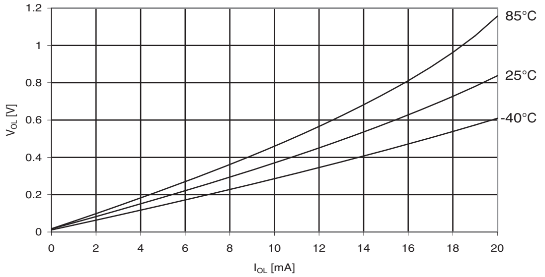
Figure 30-156. ATmega329A: I/O Pin Output Voltage vs. Sink Current, Port B ( V_{CC} = 2.7V )
