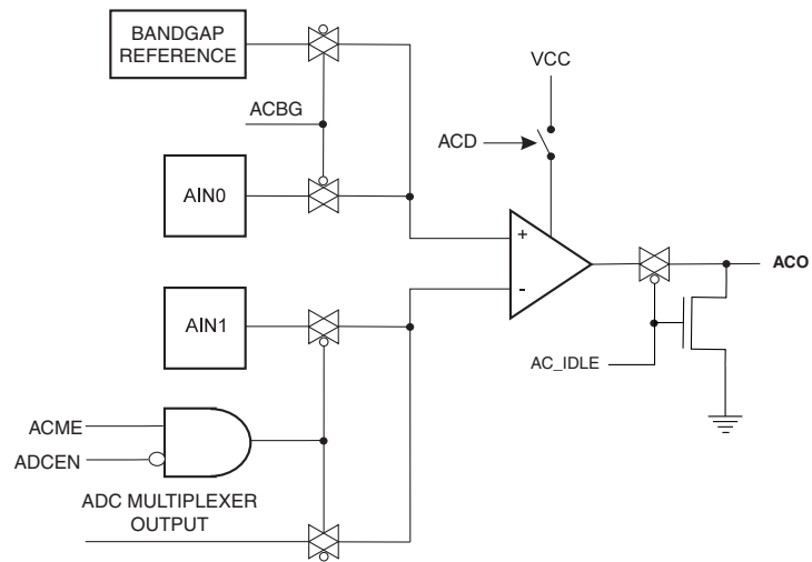
Figure 26-6. Analog Comparator
