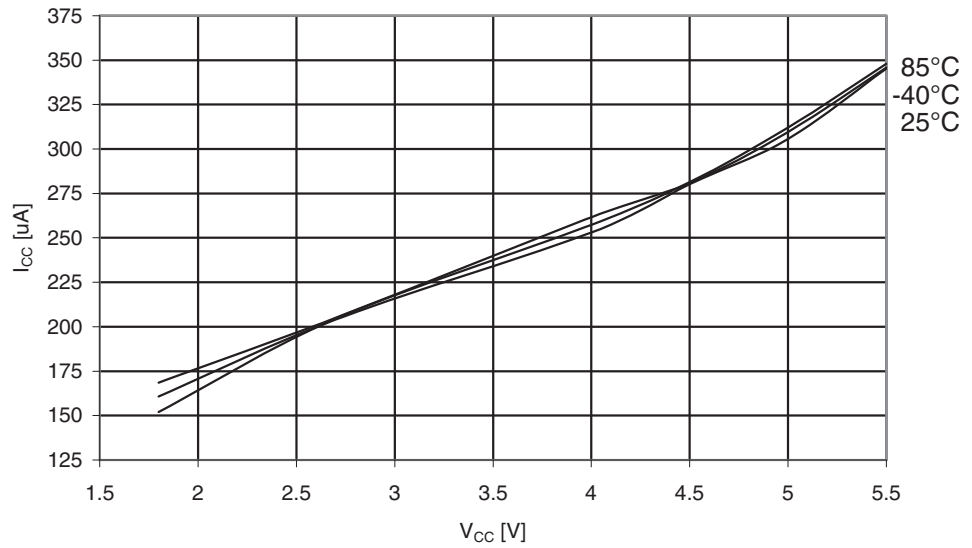
Figure 30-296. ATmega3290A: Active Supply Current with ADC at 200kHz vs. V_{CC}
