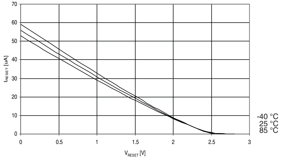
Figure 30-204. ATmega329PA: Reset Pull-up Resistor Current vs. Reset Pin Voltage ( V_{CC}=2.7V )
