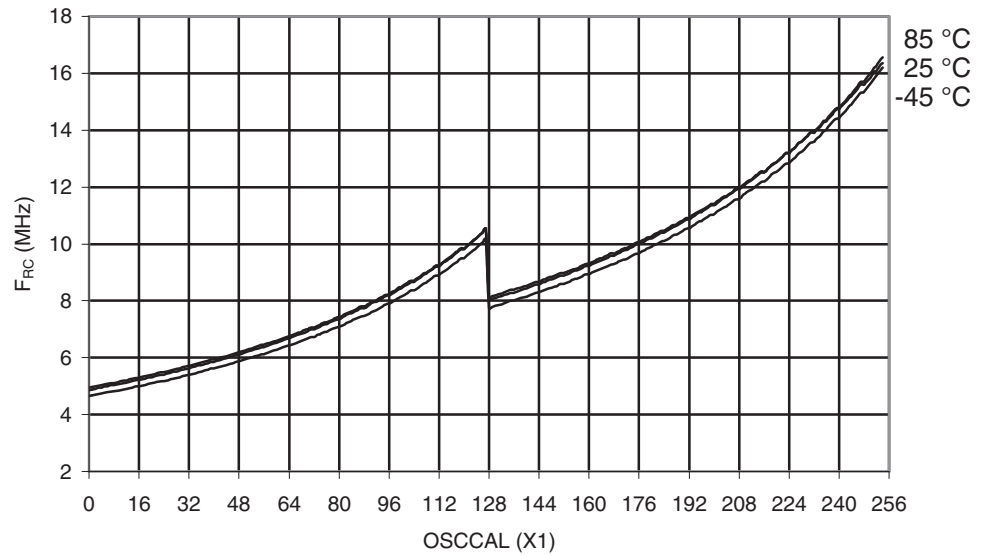
Figure 30-475. ATmega649P: Calibrated 8MHz RC Oscillator Frequency vs. OSCCAL Value
