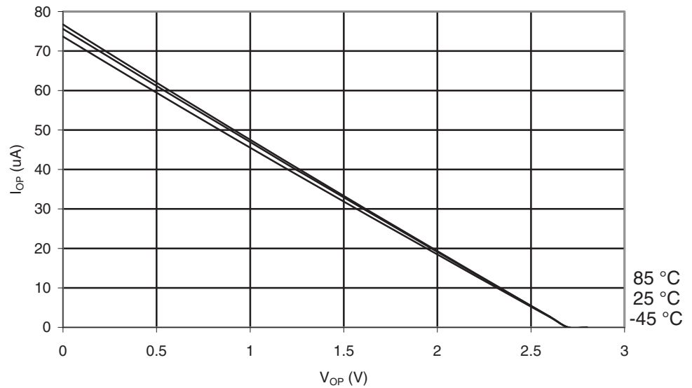
Figure 30-17. ATmega169A: I/O Pin Pull-up Resistor Current vs. Input Voltage ( V_{CC} = 2.7V )
