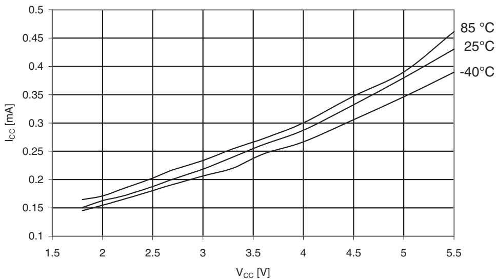
Figure 30-253. ATmega3290A: Idle Supply Current vs. V_{CC} (Internal RC Oscillator, 1MHz)
