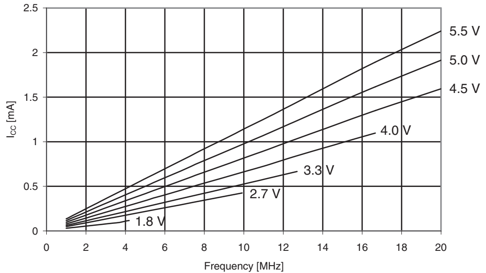
Figure 30-243. ATmega329PA: Reset Supply Current vs. V_{CC} (1 - 20MHz, Excluding Current Through The Reset Pull-up)
