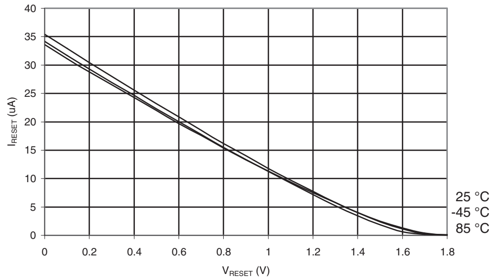
Figure 30-386. ATmega649A: Reset Pull-up Resistor Current vs. Reset Pin Voltage ( V_{CC} = 1.8V )
