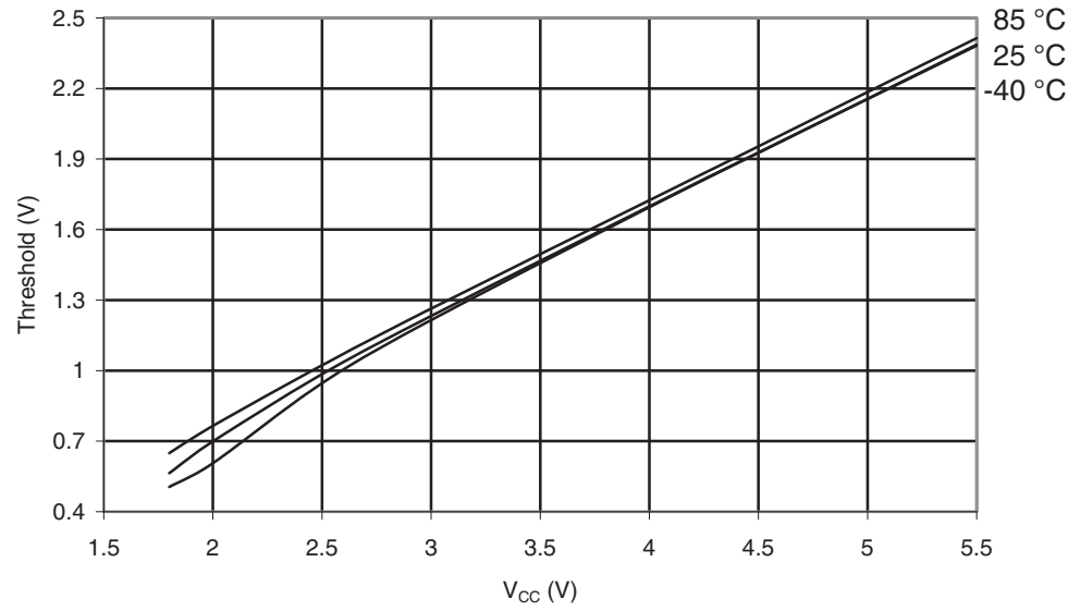
Figure 30-159. ATmega329A: I/O Pin Input Threshold Voltage vs. V_{CC} ( V_{IL} , I/O Pin Read as “0”)
