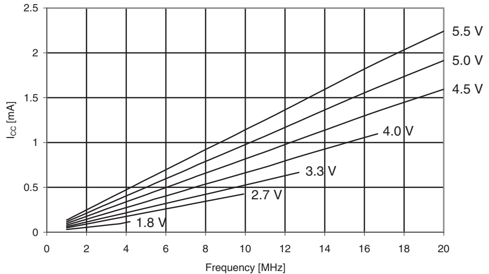
Figure 30-363. ATmega3290PA: Reset Supply Current vs. V_{CC} (1 - 20MHz, Excluding Current Through The Reset Pull-up)
