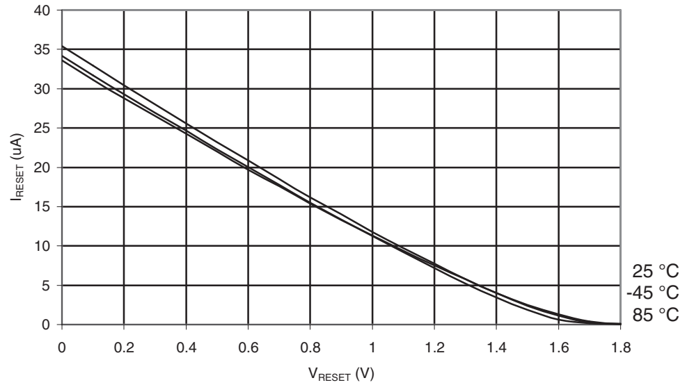
Figure 30-447. ATmega649P: Reset Pull-up Resistor Current vs. Reset Pin Voltage ( V_{CC} = 1.8V )
