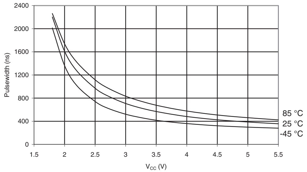
Figure 30-62. ATmega169A: Minimum Reset Pulse Width vs. V_{CC}
