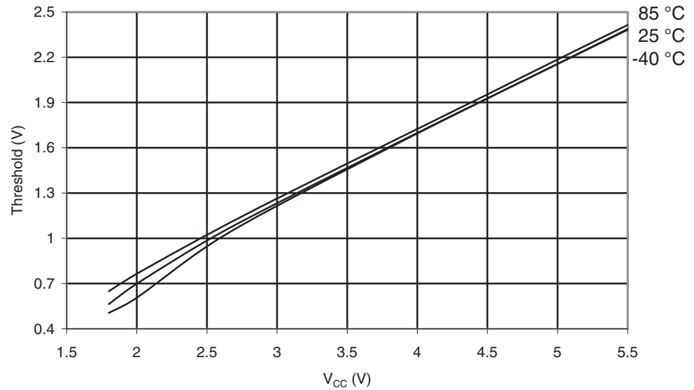
Figure 30-339. ATmega3290PA: I/O Pin Input Threshold Voltage vs. V_{CC} ( V_{IL} , I/O Pin Read as "0")
