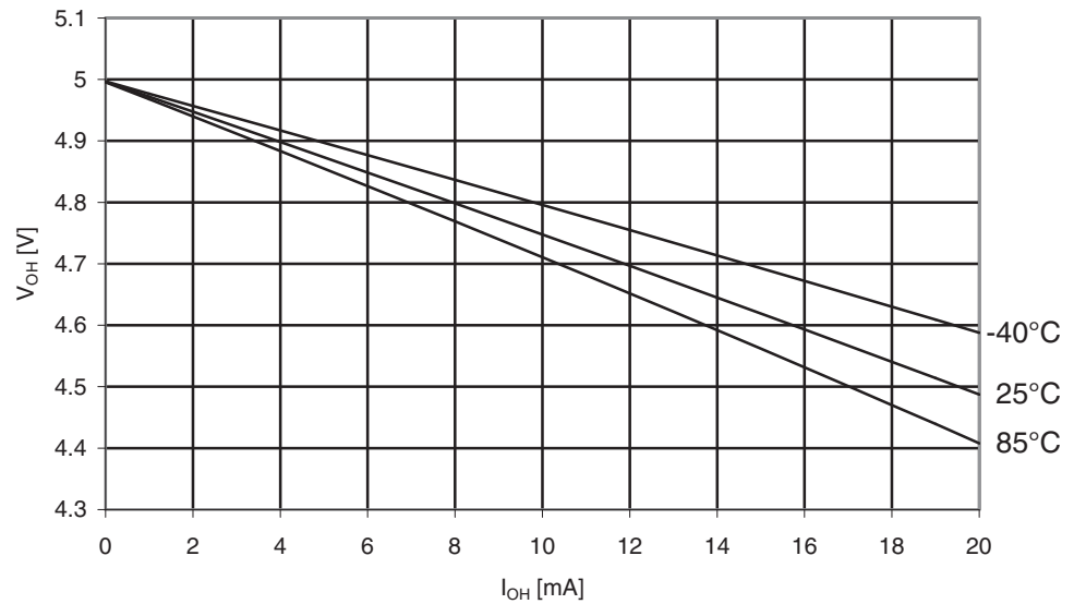
Figure 30-149. ATmega329A: I/O Pin Output Voltage vs. Source Current, Port B ( V_{CC} = 5V )
