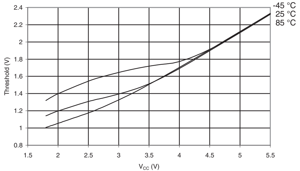
Figure 30-585. ATmega6490P: Reset Input Threshold Voltage vs. V_{CC} ( V_{IH,Reset} Pin Read as "1")
