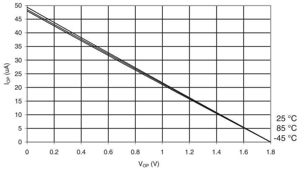
Figure 30-80. ATmega169PA: I/O Pin Pull-up Resistor Current vs. Input Voltage ( V_{CC} = 1.8V )
