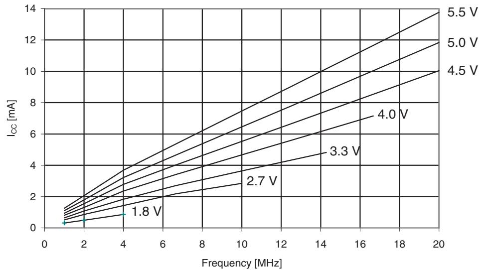
Figure 30-246. ATmega3290A: Active Supply Current vs. Frequency (1 - 20MHz)
