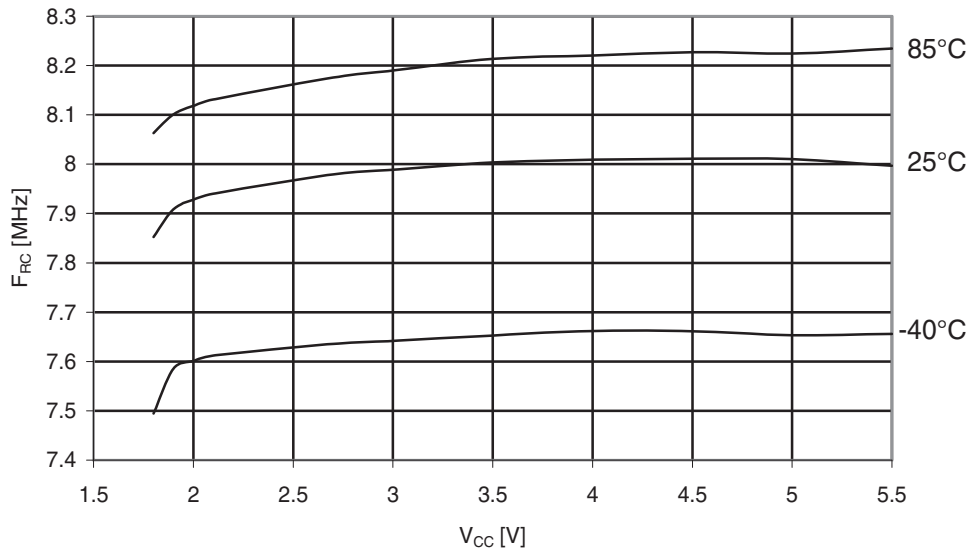
Figure 30-172. ATmega329A: Calibrated 8MHz RC Oscillator Frequency vs. V_{CC}
