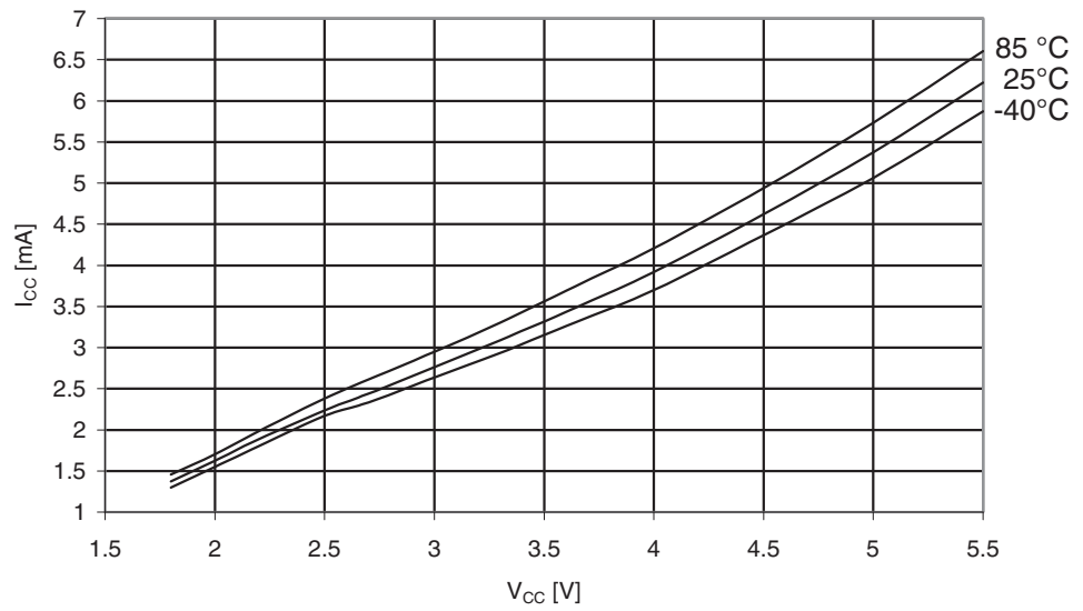
Figure 30-127. ATmega329A: Active Supply Current vs. V_{CC} (Internal RC Oscillator, 8MHz)
