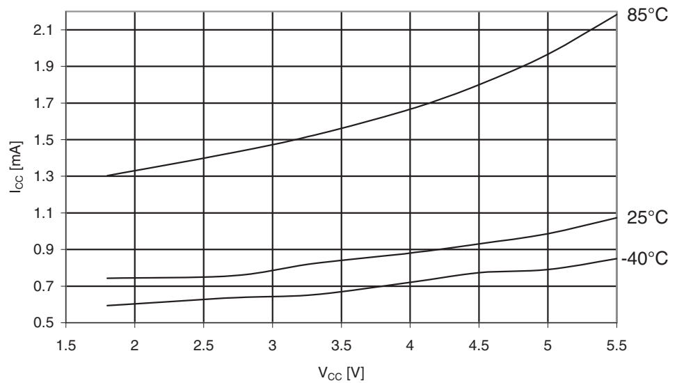
Figure 30-258. ATmega3290A: Standby Supply Current vs. V_{CC} (32kHz Watch Crystal, Watchdog Timer Disabled)
