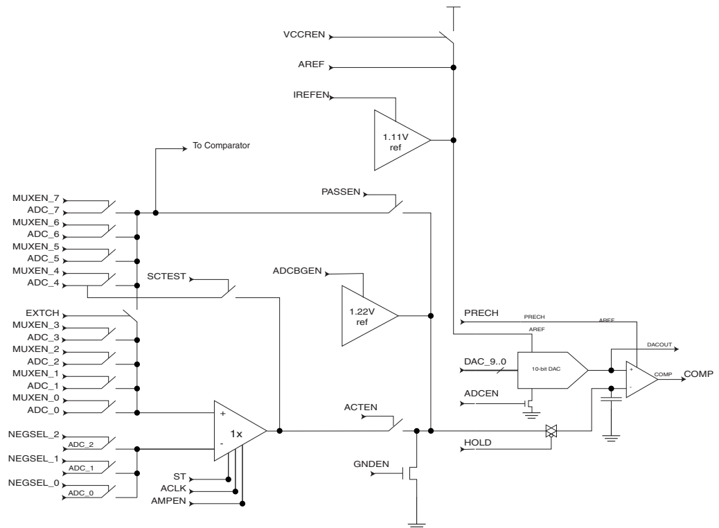
Figure 26-8. Analog to Digital Converter
