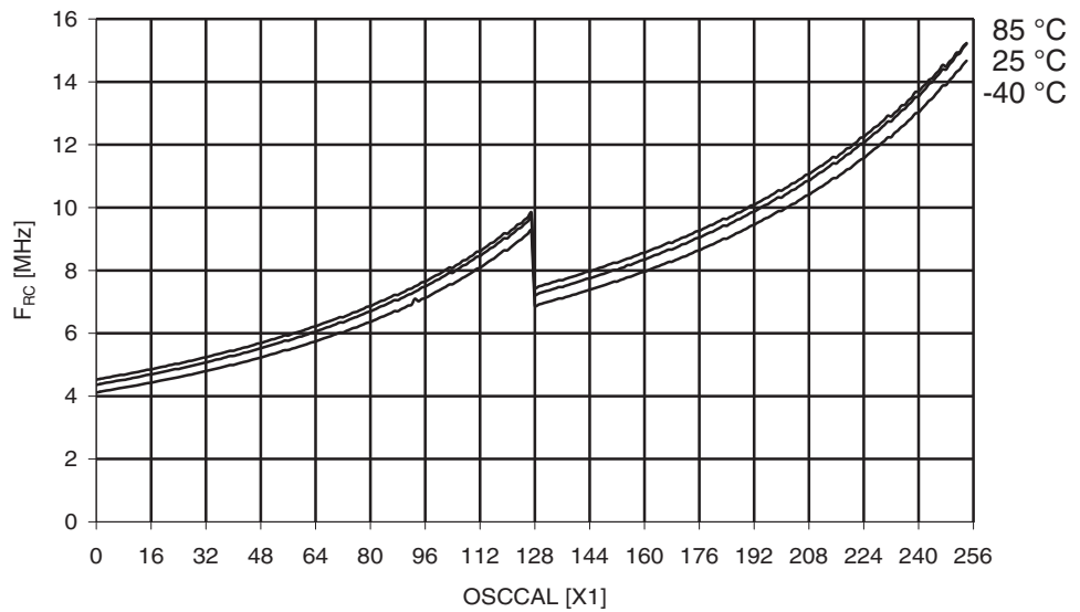
Figure 30-173. ATmega329A: Calibrated 8MHz RC Oscillator Frequency vs. Oscscal Value
