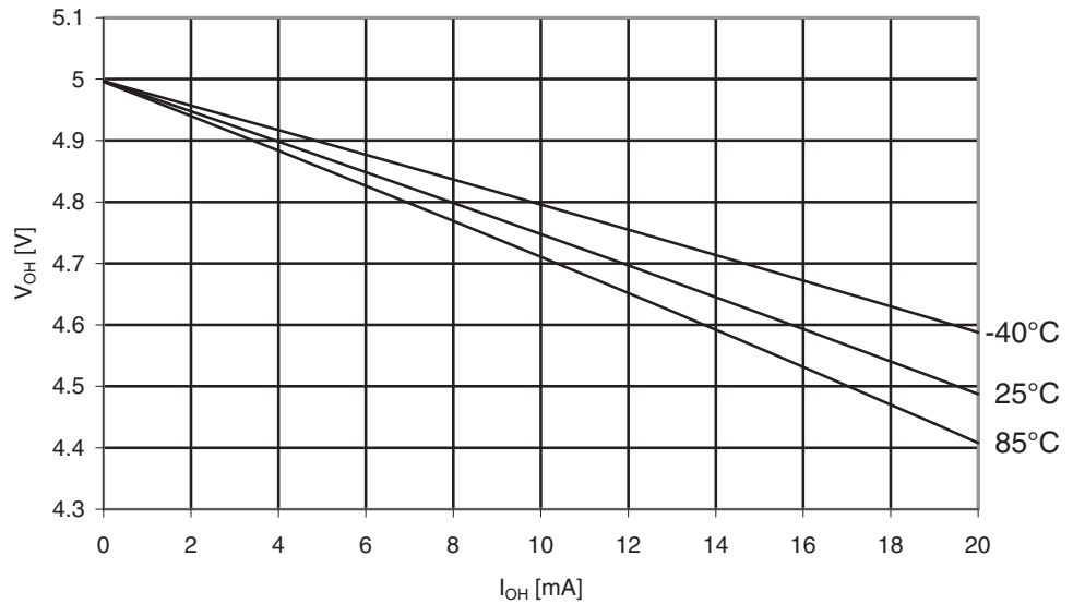
Figure 30-209. ATmega329PA: I/O Pin Output Voltage vs. Source Current, Port B ( V_{CC} = 5V )
