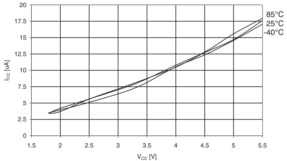
Figure 30-359. ATmega3290PA: Watchdog Timer Current vs. V_{CC}
