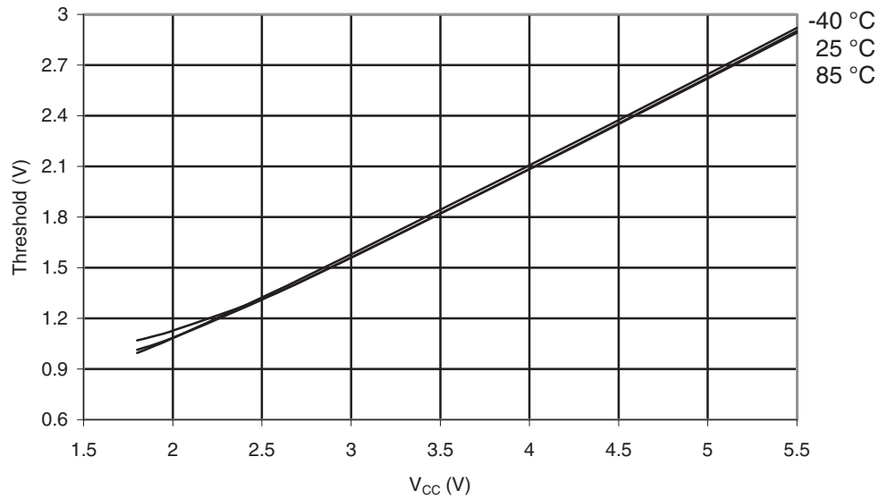
Figure 30-338. ATmega3290PA: I/O Pin Input Threshold Voltage vs. V_{CC} ( V_{IH} , I/O Pin Read as "1")
