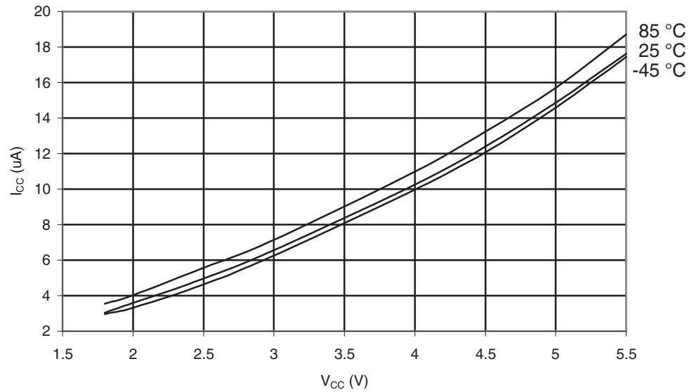
Figure 30-437. ATmega649P: Power-down Supply Current vs. V_{CC} (Watchdog Timer Enabled)
