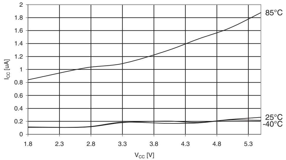
Figure 30-196. ATmega329PA: Power-down Supply Current vs. V_{CC} (Watchdog Timer Enabled)
