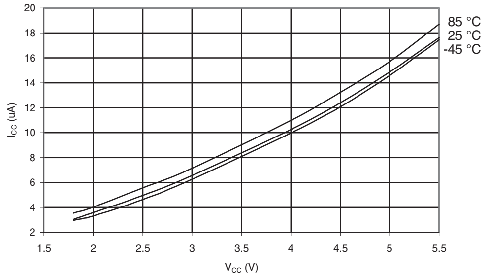
Figure 30-559. ATmega6490P: Power-down Supply Current vs. V_{CC} (Watchdog Timer Enabled)
