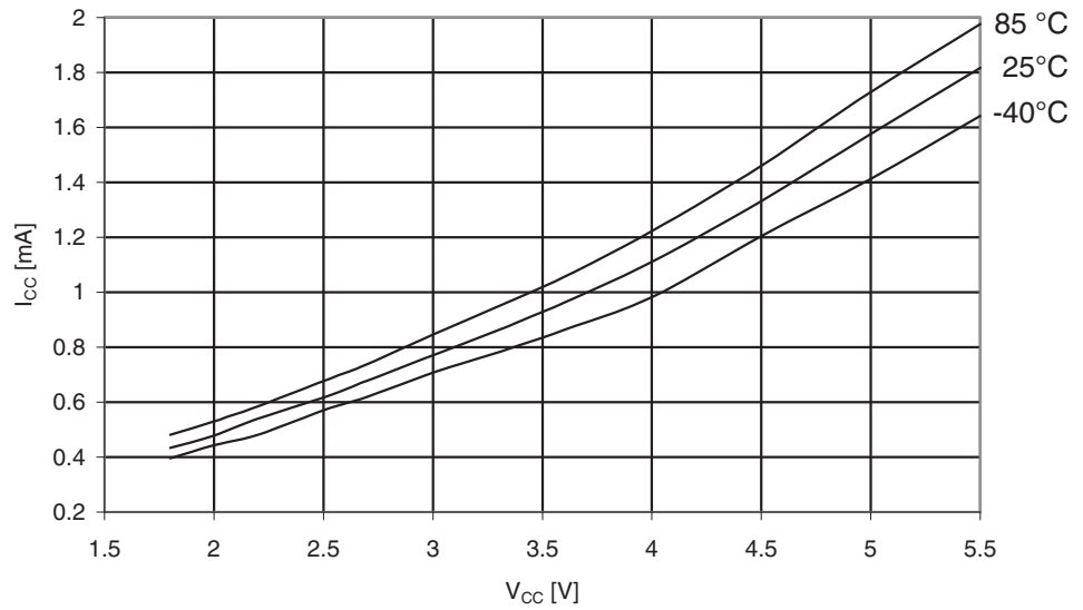
Figure 30-192. ATmega329PA: Idle Supply Current vs. V_{CC} (Internal RC Oscillator, 8MHz)
