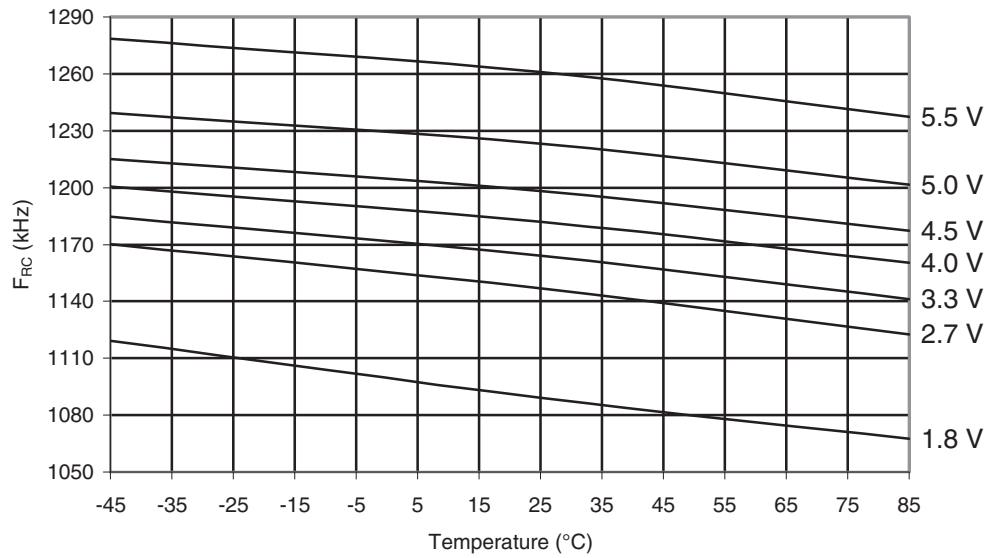
Figure 30-472. ATmega649P: Watchdog Oscillator Frequency vs. Temperature
