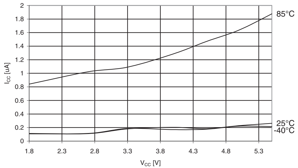
Figure 30-256. ATmega3290A: Power-down Supply Current vs. V_{CC} (Watchdog Timer Enabled)
