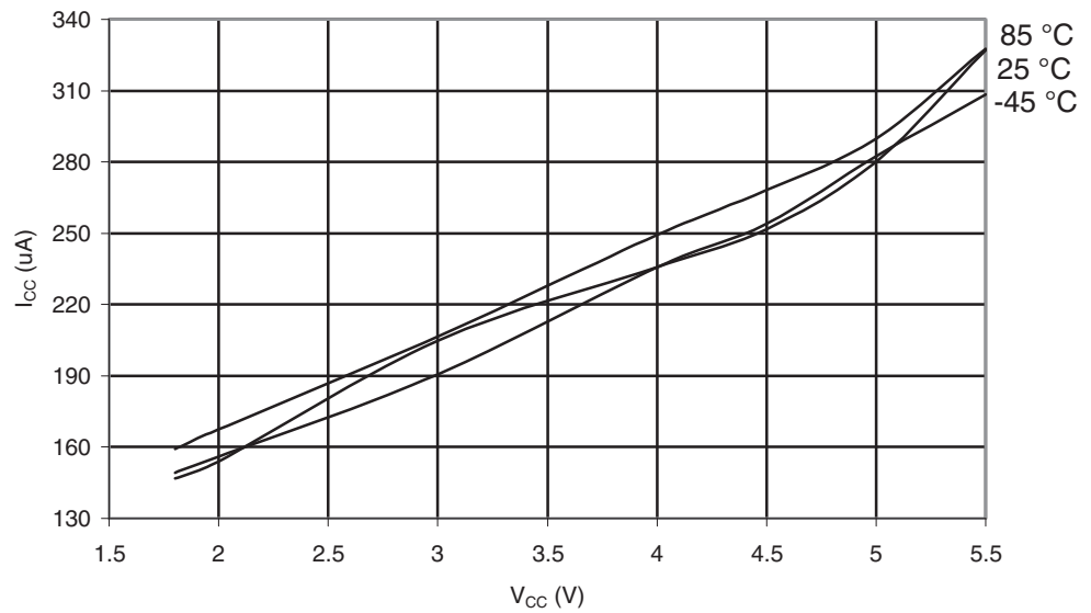
Figure 30-540. ATmega6490A: Active Supply Current with ADC at 1MHz vs. V_{CC}
