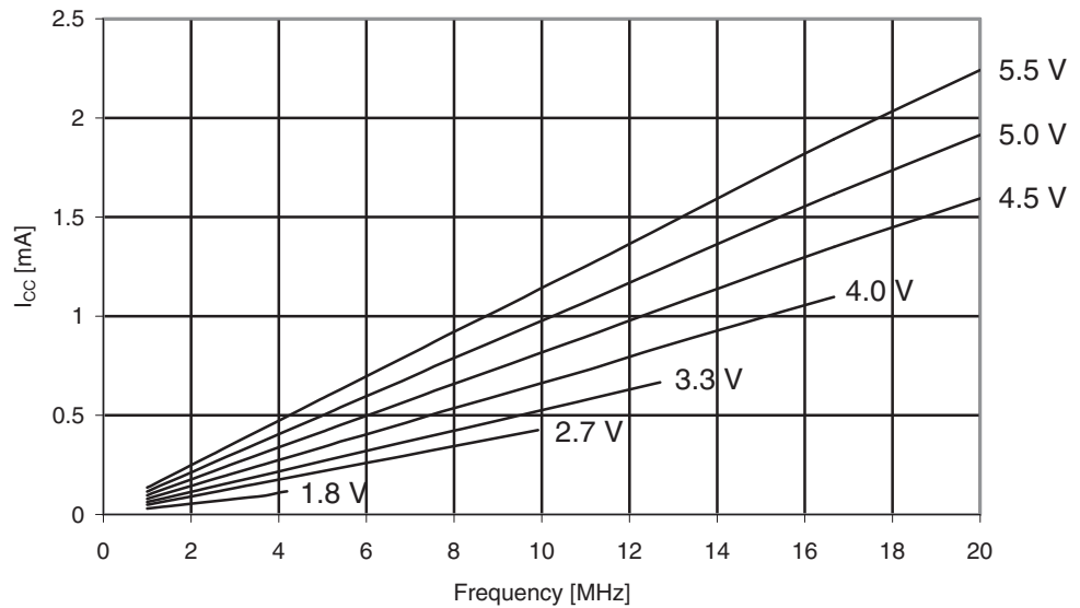
Figure 30-183. ATmega329A: Reset Supply Current vs. V_{CC} (1 - 20MHz, Excluding Current Through The Reset Pull-up)
