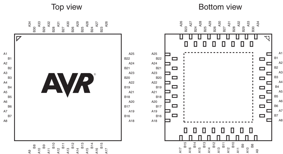
Figure 1-3. Pinout ATmega169A/ATmega169PA
