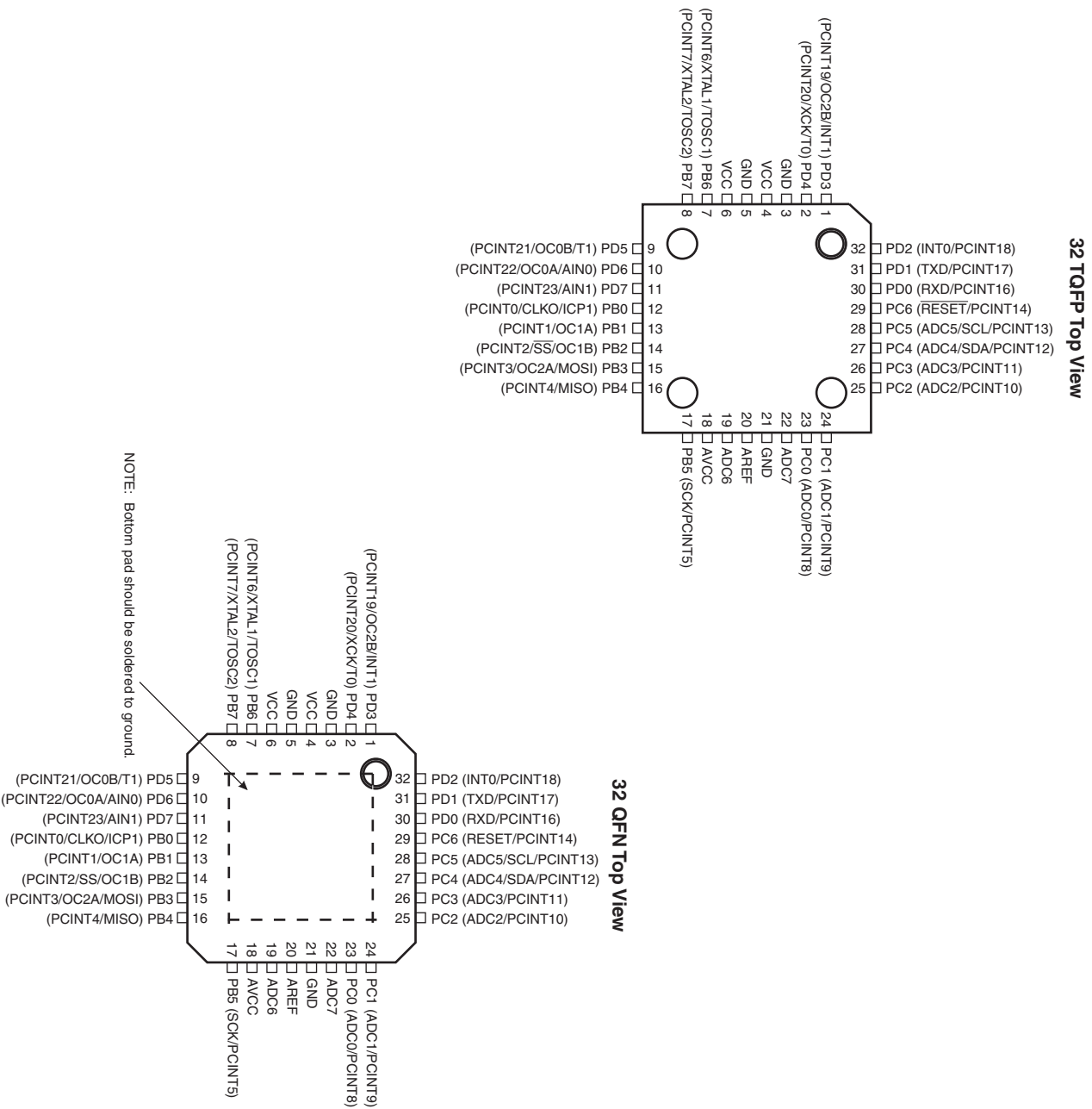
Figure 1-1. Pinout Atmel® ATmega48PA/88PA/168PA
