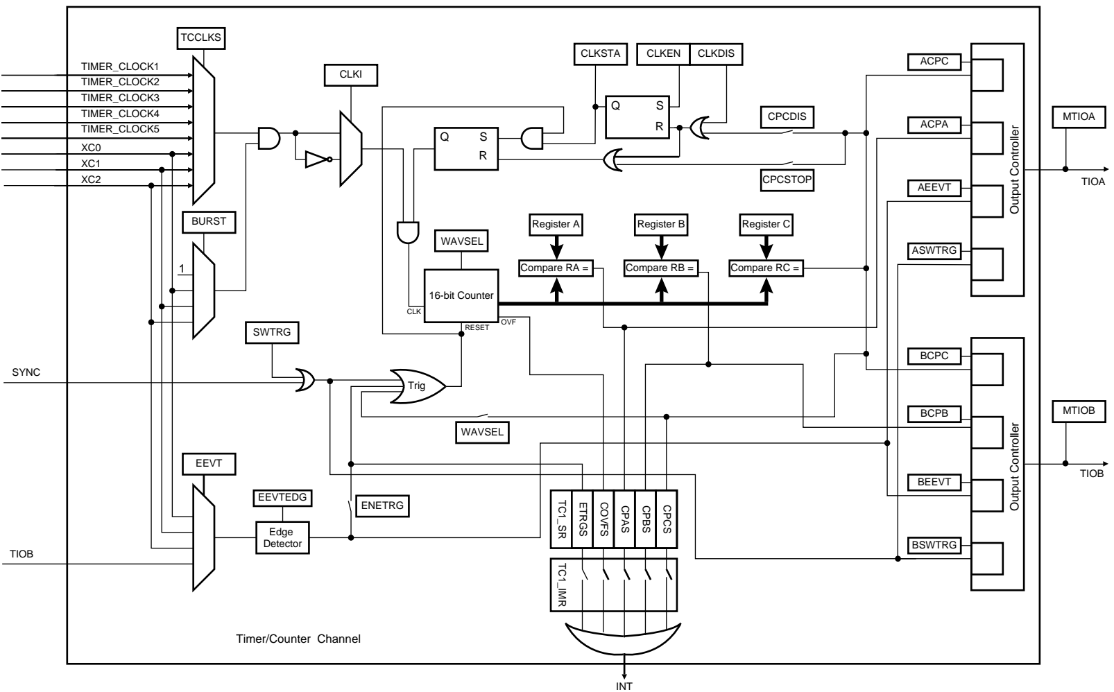
Figure 36-6. Waveform Mode
