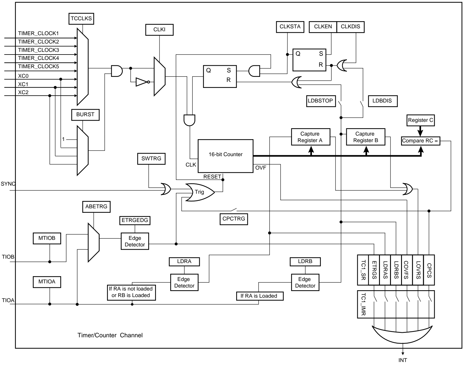
Figure 36-5. Capture Mode
