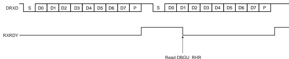
Figure 30-5. Receiver Ready
