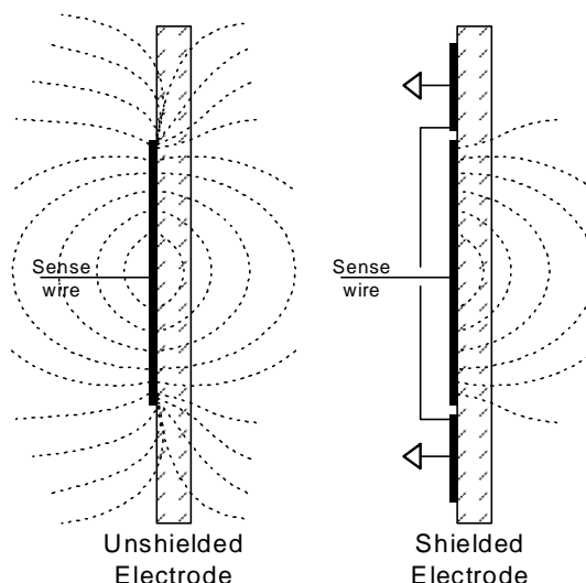
Figure 2-3. Shielding Against Fringe Fields
