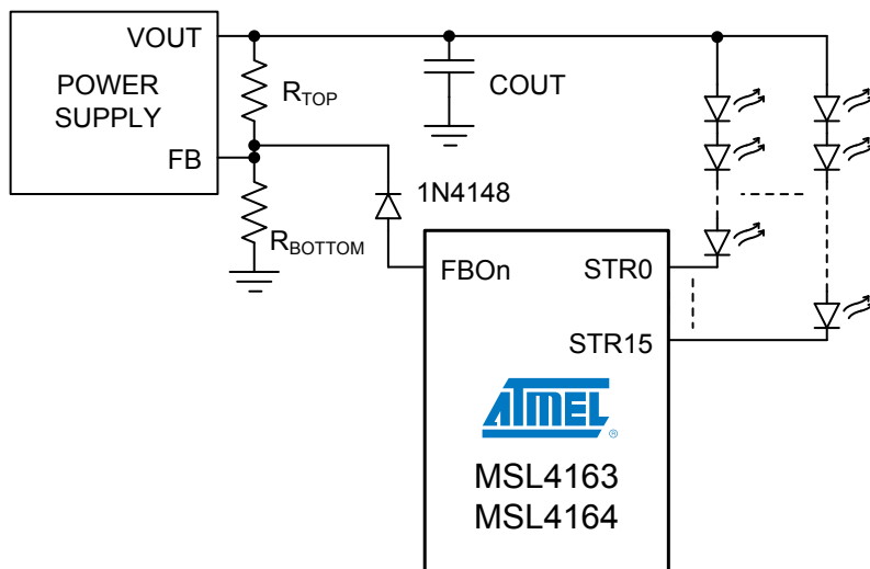
Figure 6. FBO n Connects to the Power Supply Voltage Divider through a Diode.
