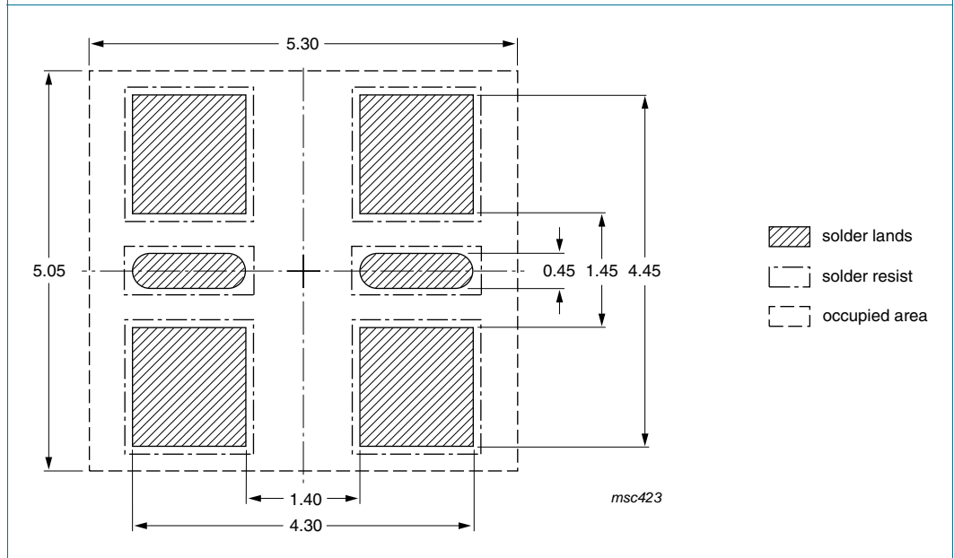
Fig 15. Reflow soldering footprint SOT457 (SC-74)
