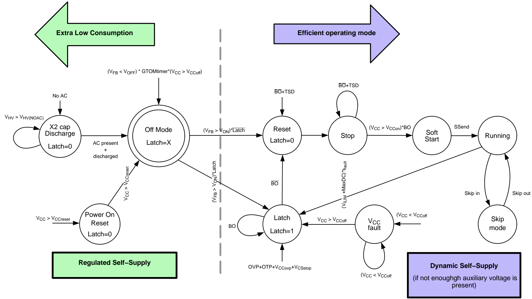
Figure 46. Operating Status Diagram for the Fully Latched Version A of the Device
