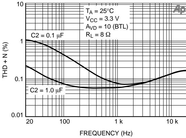
Figure 10. THD + N vs. Frequency (P L = 350 mW)
