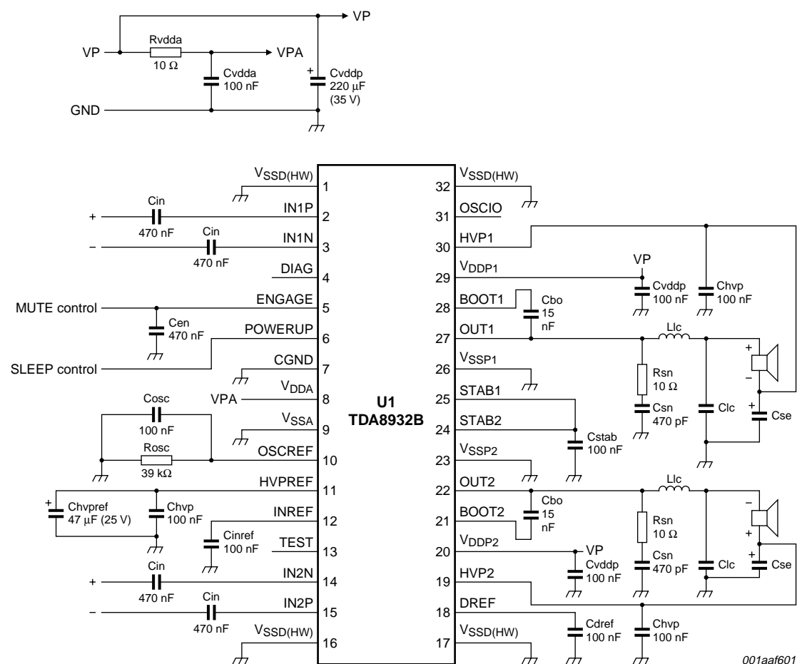
Fig 36. Typical simplified application diagram for 2 \times \text{SE} (asymmetrical supply)
