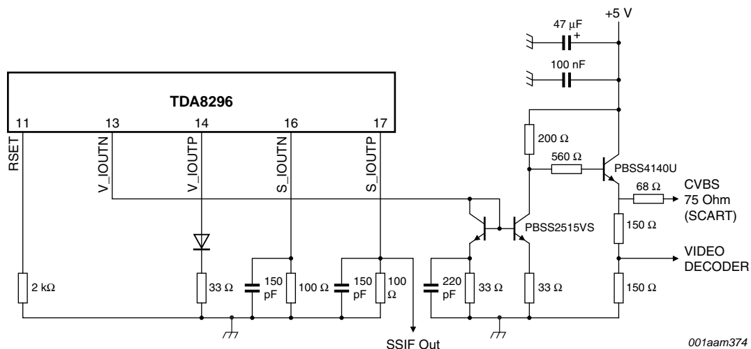
Fig 25. Buffer application with 75 \Omega load
