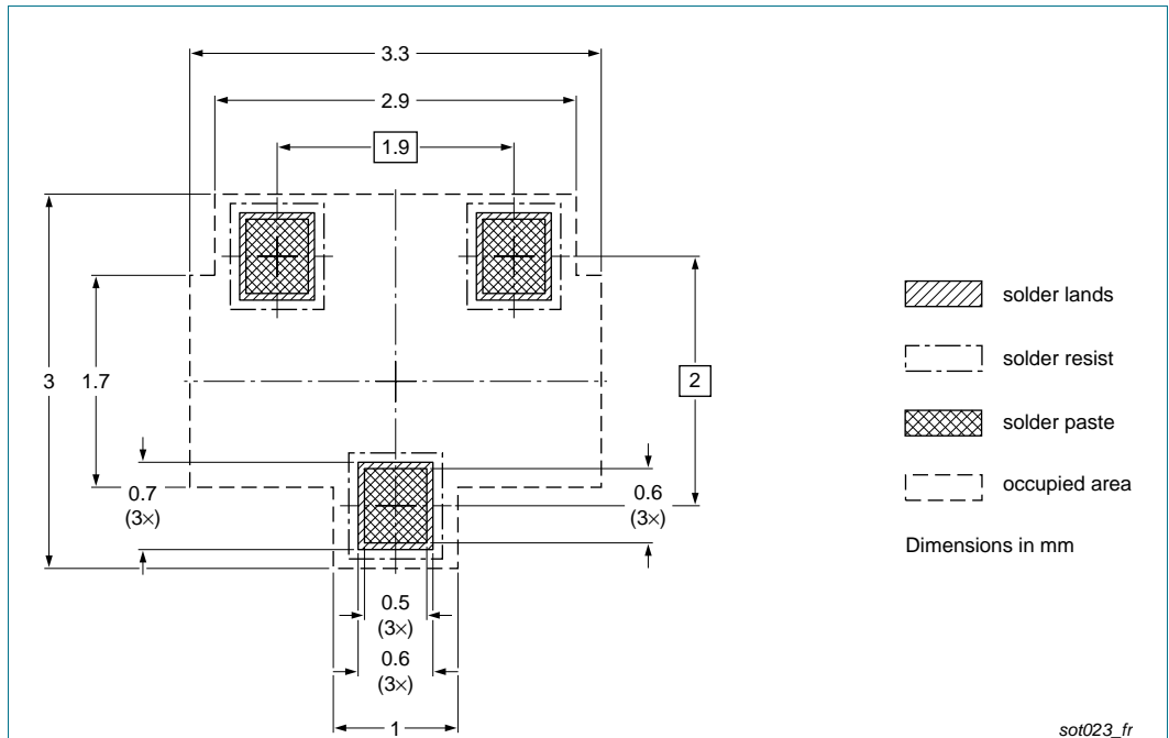
Fig 18. Reflow soldering footprint PDTC114ET (SOT23)
