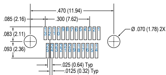
25 Contacts
