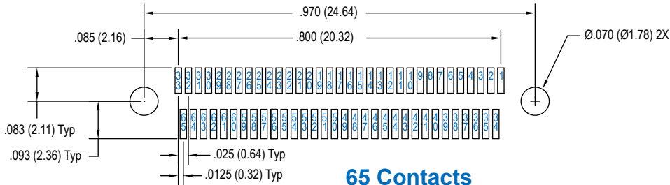
65 Contacts
