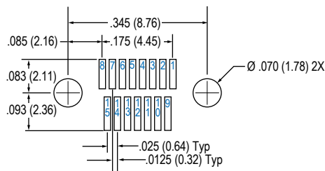
15 Contacts
