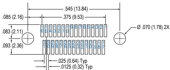
31 Contacts
