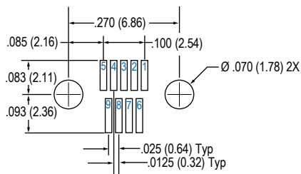
9 Contacts
