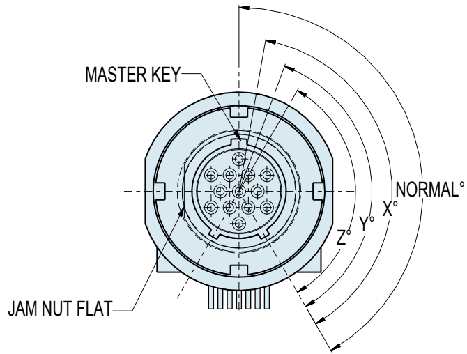
JAM NUT FLAT AND KEYWAY LOCATIONS SHELL SIZE 5 AND 6 SOCKET FACE SHOWN
