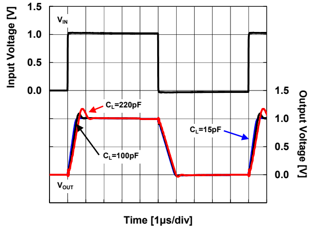
Pulse Response
