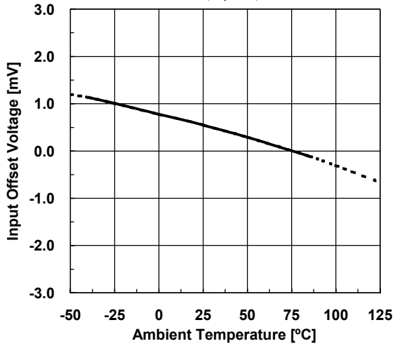
Input Offset Voltage vs. Temperature V^+/V^-=\pm 2.5V, G_v=0dB, T_a=25^\circ C
