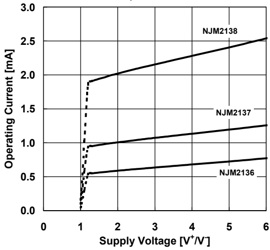
Operating Current vs. Supply Voltage G_v=0dB, T_a=25^\circ C
