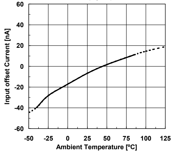
Input Offset Current vs. Temperature V^+/V^-=\pm 2.5V, G_v=0dB, T_a=25^\circ C
