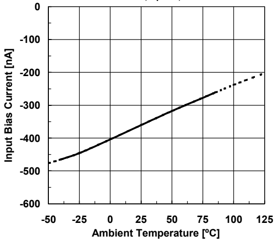
Input Bias Current vs. Temperature V^+/V^-=\pm 2.5V, G_v=0dB, T_a=25^\circ C
