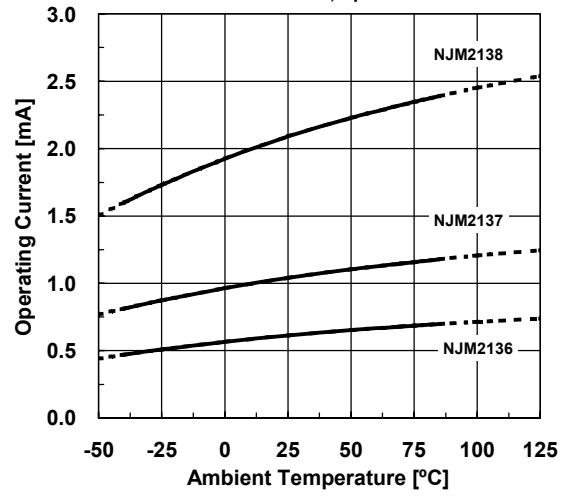
Operating Current vs. Temperature V^+/V^-=\pm 2.5V, G_v=0dB
