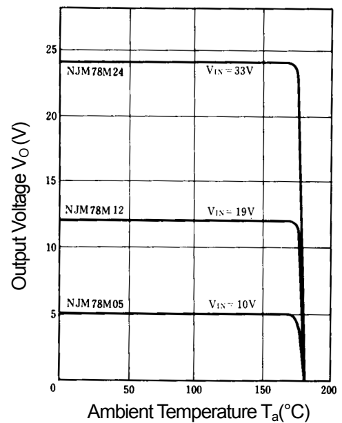
Thermal Shutdown Characteristics
