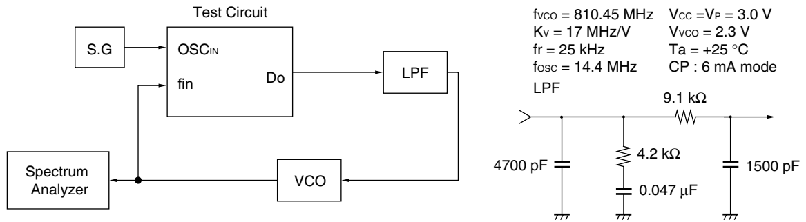
PLL Reference Leakage
