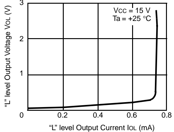
Fig. 27 -"L" level Output Voltage vs. "L" level Output Current
