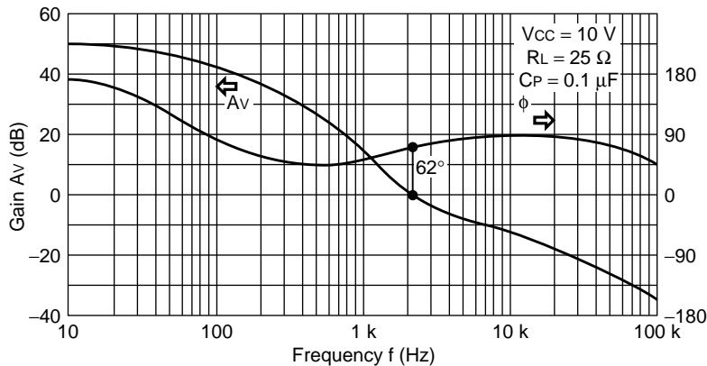
Figure 38 DC/DC Converter +5 V output Gain vs. Phase
