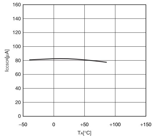
I_{CCSCR} - T_A V_{CC} = 3.0\text{ V} , F_{MPL} = 50\text{ kHz} (divided by 2) Subclock mode with the sub-CR clock operating
