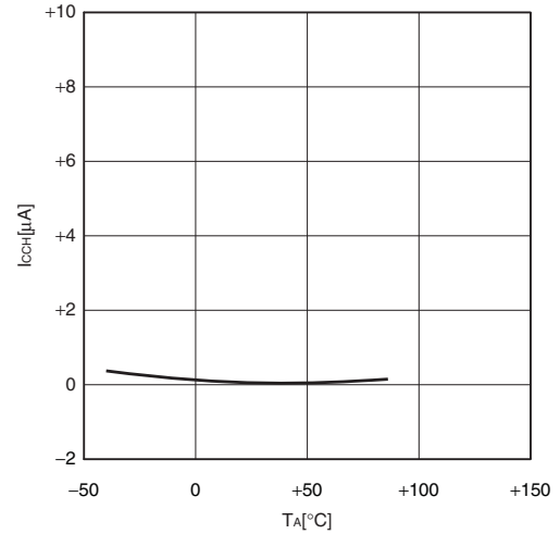
I_{CCH} - T_A V_{CC} = 3.0\text{ V} , F_{MPL} = (\text{stop}) Substop mode with the external clock stopping
