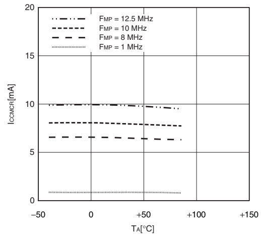
I_{CCMCR} - T_A V_{CC} = 3.0\text{ V} , F_{MP} = 1, 8, 10, 12.5\text{ MHz} (no division) Main clock mode with the main CR clock operating
