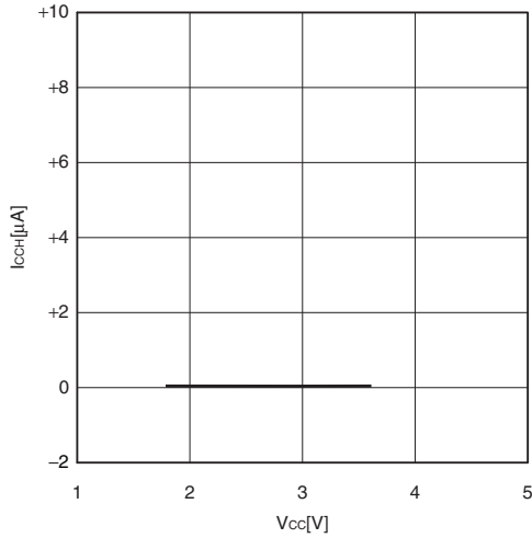
I_{CCH} - V_{CC} T_A = +25^\circ\text{C} , F_{MPL} = (\text{stop}) Substop mode with the external clock stopping
