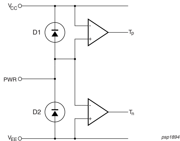
Fig.3 OM1894 power supply circuit
