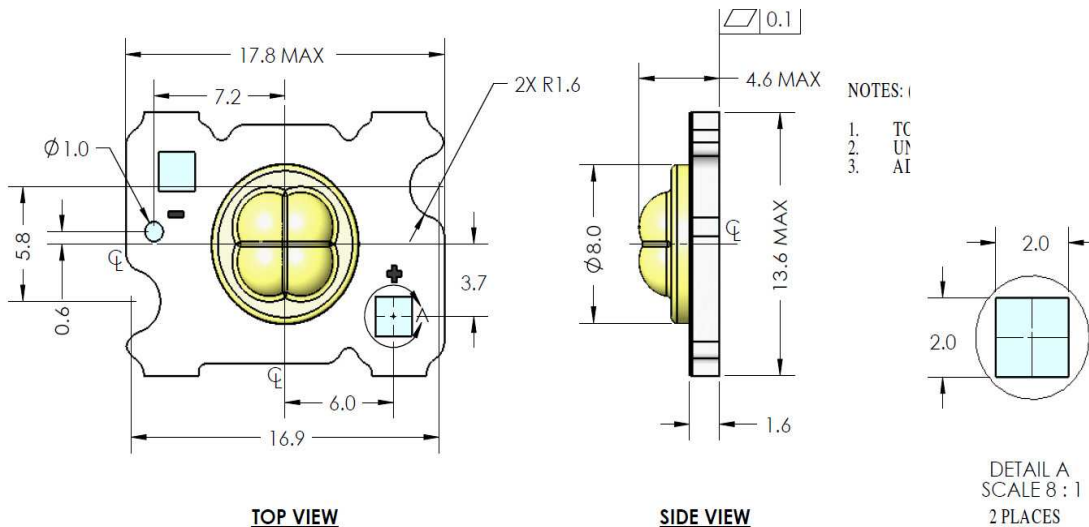
Figure 1: Drawing for all BXRB LS Array parts.
