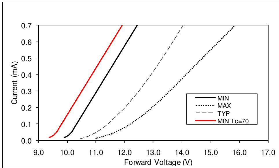
Figure 11: Typical Current vs. Voltage, BXR-XXX0360-A-00, BXR-XXX0470-A-00
