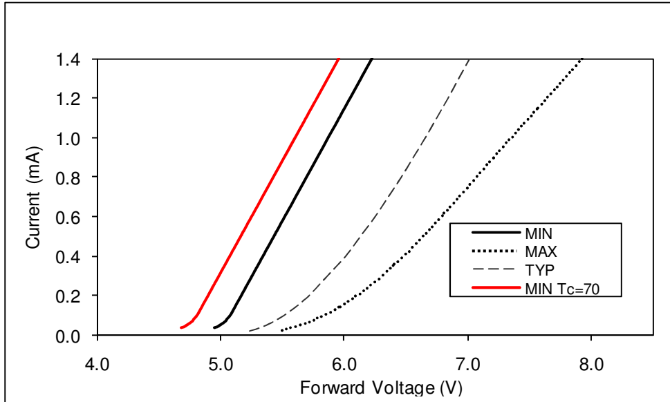
Figure 10: Typical Current vs. Voltage, BXR-XXX0360-B-00, BXR-XXX0470-B-00
