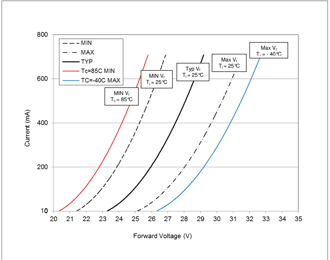
Figure 1: Electrical Characteristics
