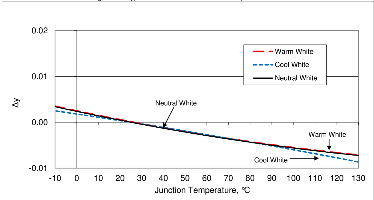
Figure 4: Typical ccx Shift vs. Junction Temperature
