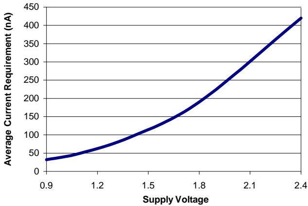
Average Supply Current vs. Supply Voltage, 25°C AHL0xx-14E
