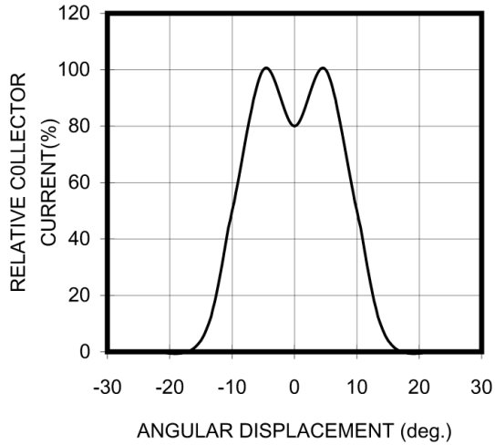
ANGULAR DISPLACEMENT
