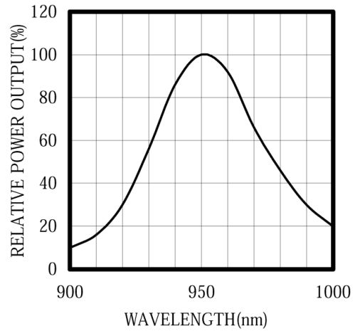
SPECTRAL OUTPUT
