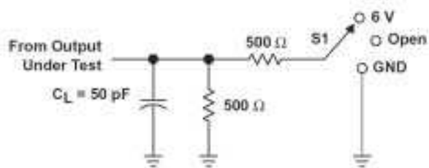
FIGURE 1. LOAD CIRCUIT
