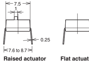
Raised actuator
