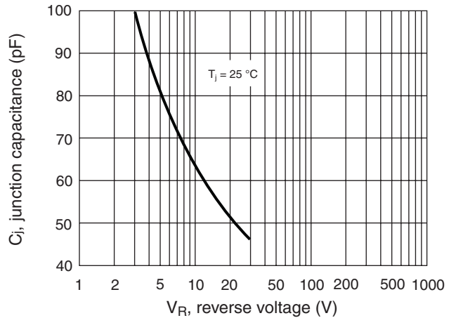
TYPICAL JUNCTION CAPACITANCE PER DIODE
