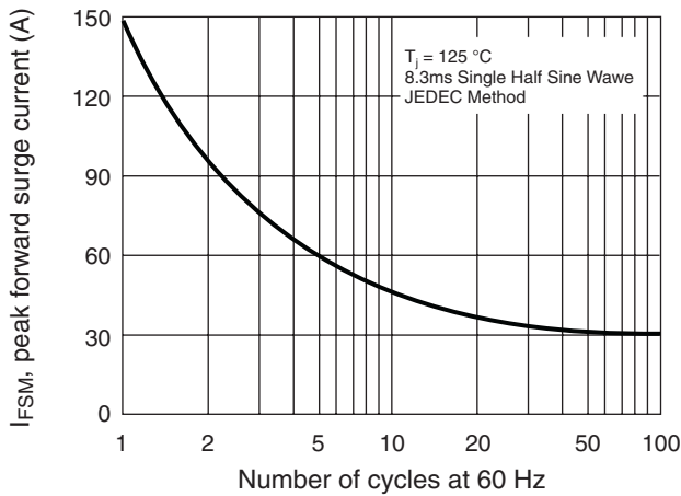
MAXIMUM NON-REPETITIVE FORWARD SURGE CURRENT PER DIODE
