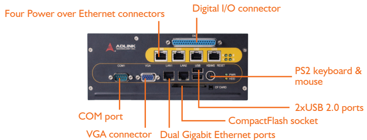
EOS-1000 Front View
