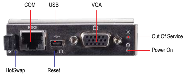
Front Panel I/O Interfaces Front Panel LED Indicators and Reset
