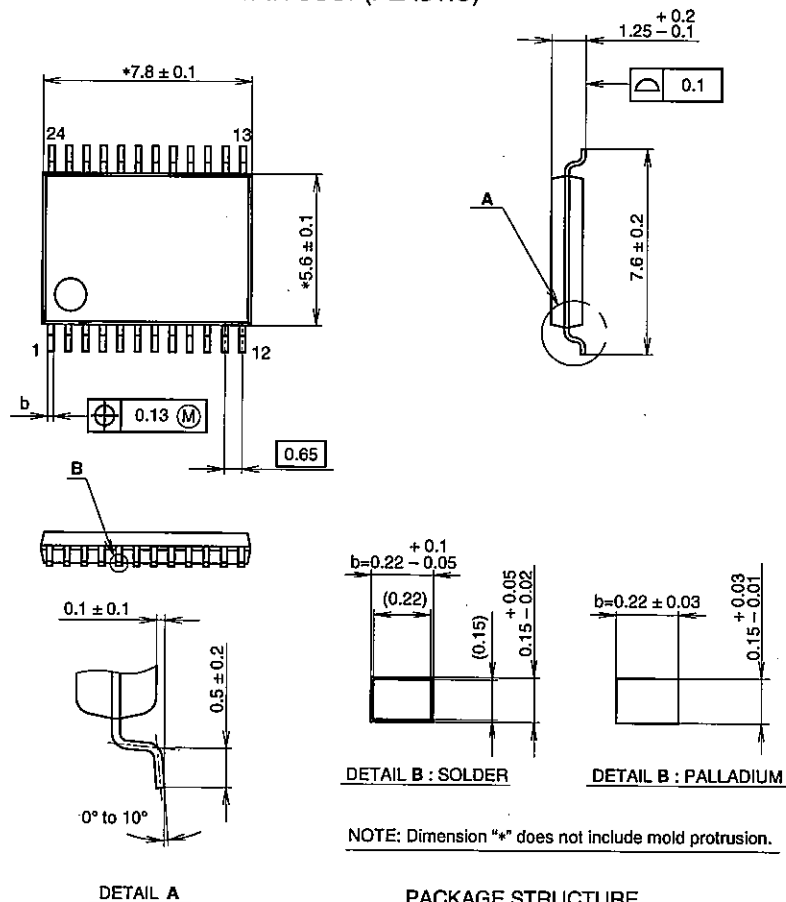
DETAIL A
