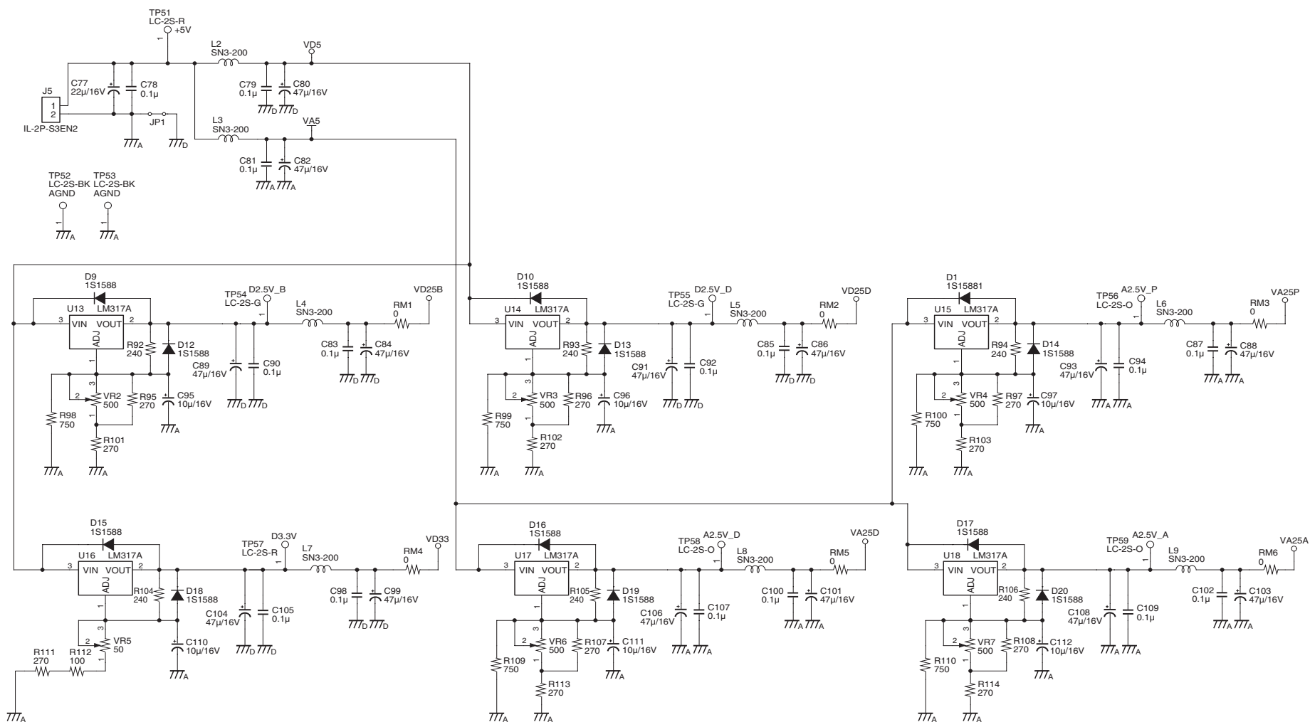
CXD4016R EVB Circuit Diagram (POWER)
