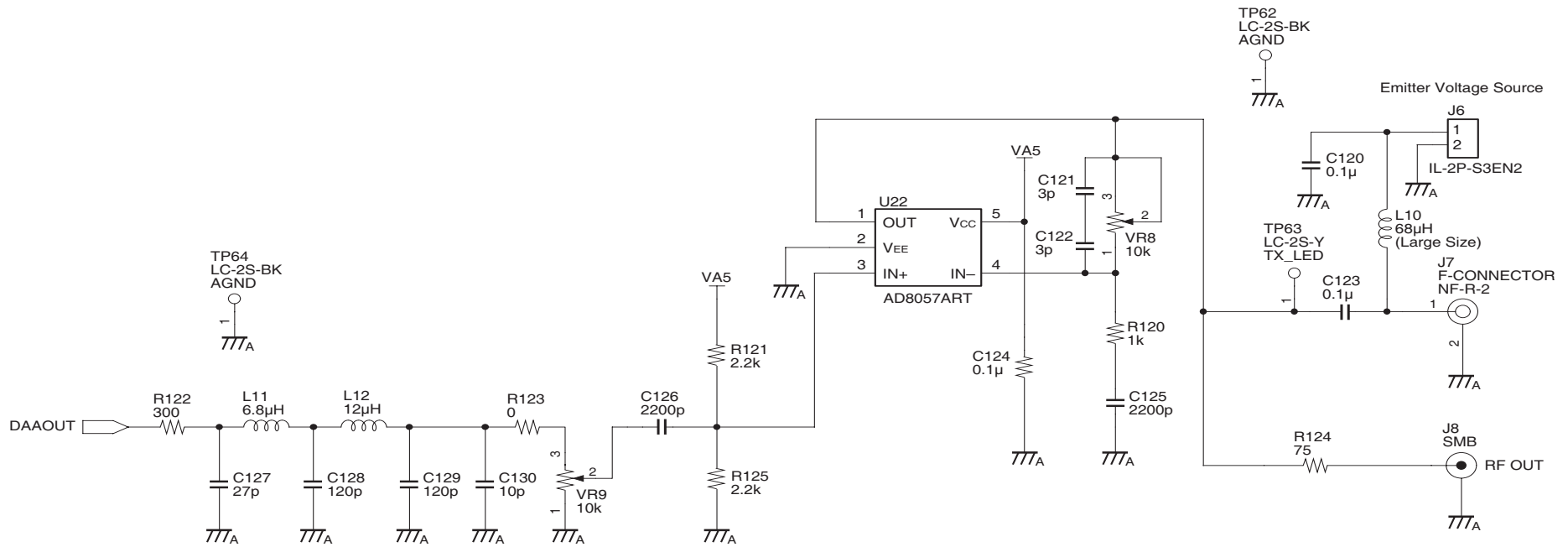
CXD4016R EVB Circuit Diagram (RFOUT)
