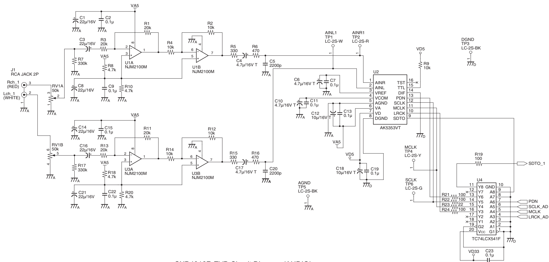
CXD4016R EVB Circuit Diagram (AUDIO)
