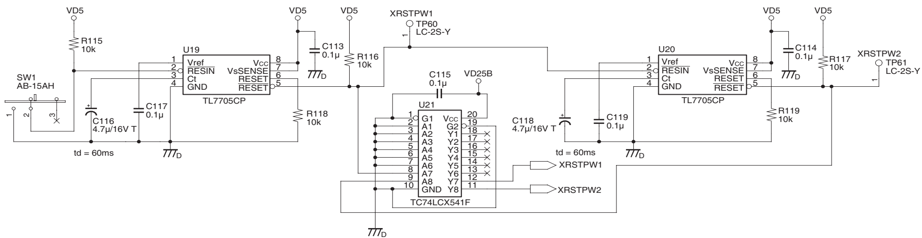
CXD4016R EVB Circuit Diagram (RESET)
