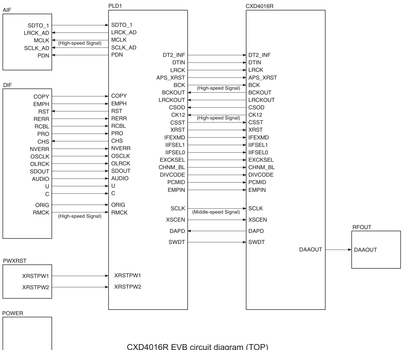
CXD4016R EVB circuit diagram (TOP)
