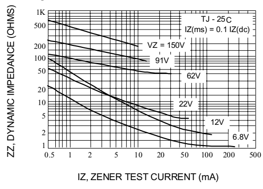
Fig. 4-EFFECT OF ZENER CURRENT
