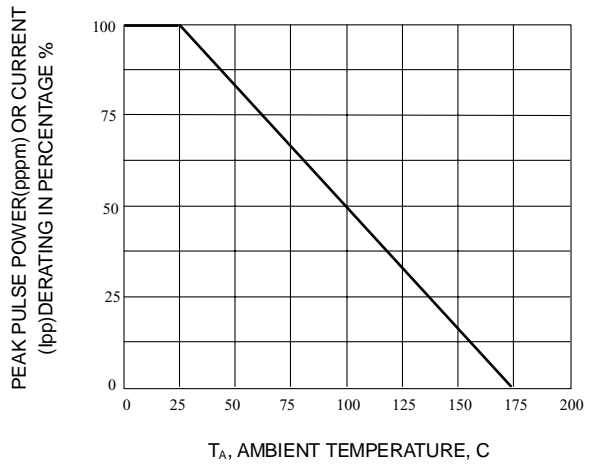
Fig. 2-PULSE DERATING CURVE
