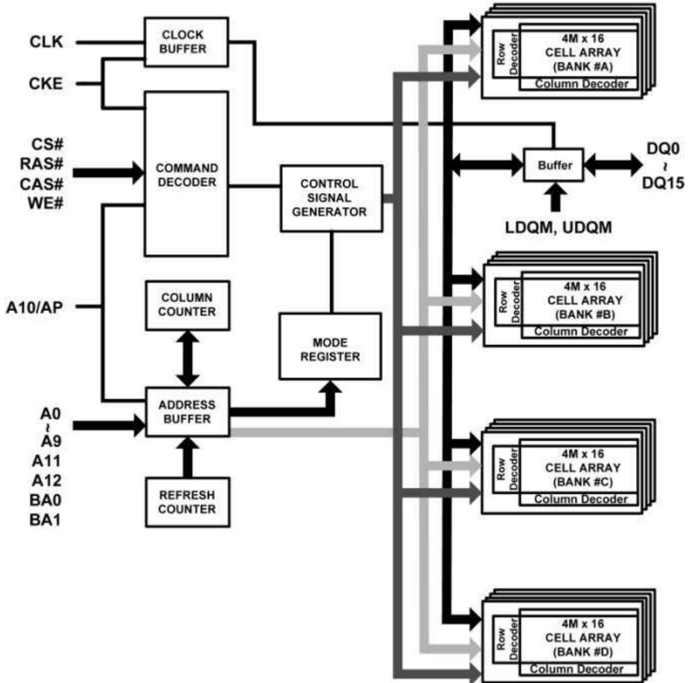
Figure 2. Block Diagram
