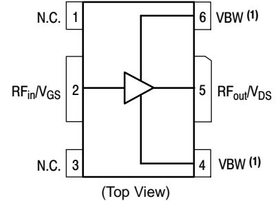
Figure 1. Pin Connections
