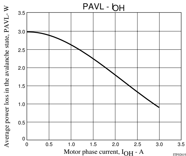
Figure 3 Allowable Loss Range, PAVL-I OH During STK672-220-E Avalanche Operations
