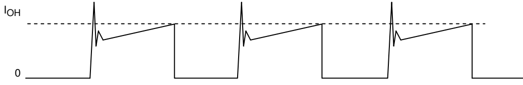
Model of the Motor Current Flowing into the Driver IC (pins 2, 3, 4, and 5)
