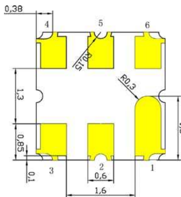
Figure 4 Bottom View
