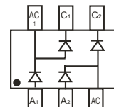
CDBV6-54BR-G Marking: KLB
