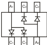
CDBV6-54AD-G* Marking: KL6
