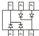
CDBV6-54CD-G* Marking: KL7
