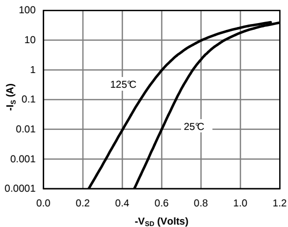
Figure 17: Body-Diode Characteristics
