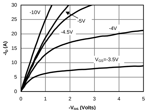
Fig 12: On-Region Characteristics
