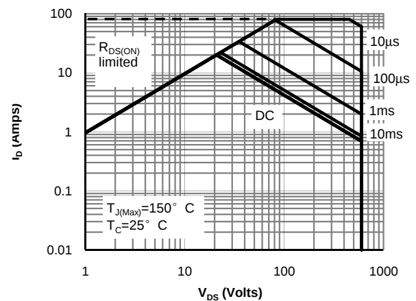
Figure 10: Maximum Forward Biased Safe Operating Area for AOK20N60 (Note F)
