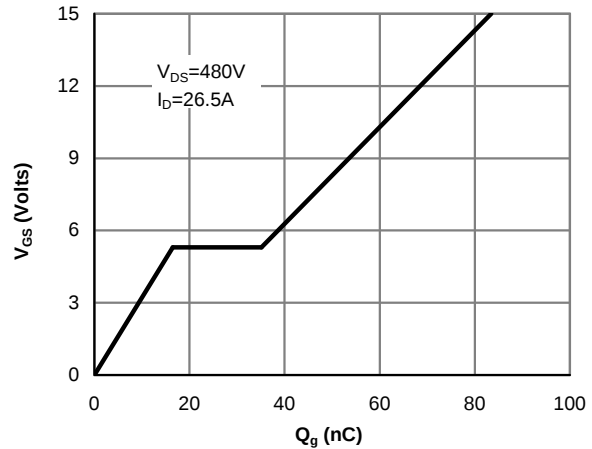
Figure 8: Gate-Charge Characteristics
