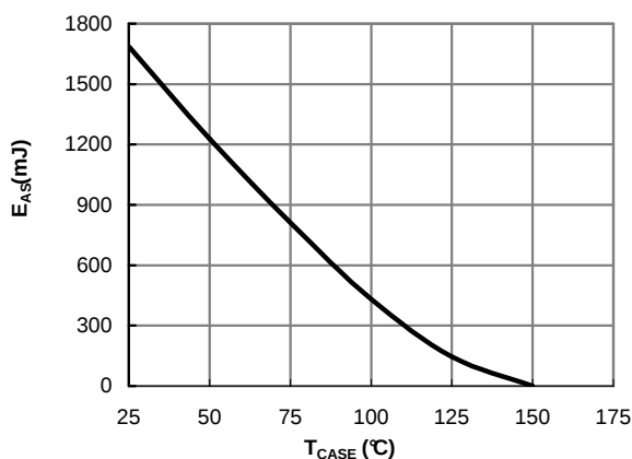
Figure 12: Avalanche energy
