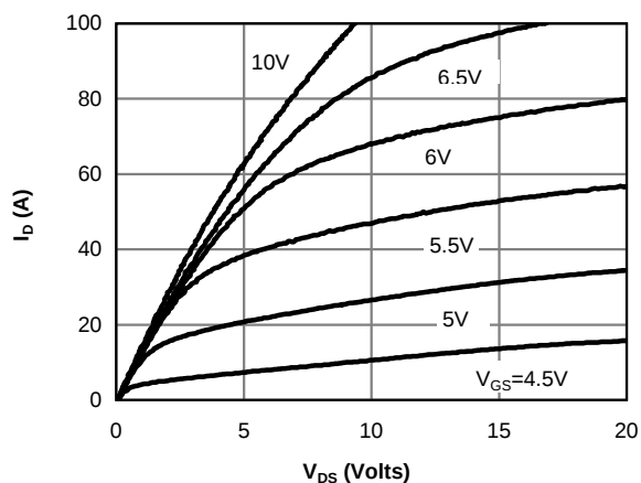
Figure 1: On-Region Characteristics@25°C
