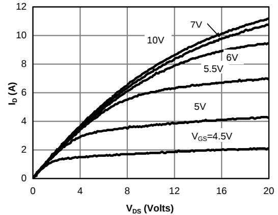
Figure 2: On-Region Characteristics@125°C
